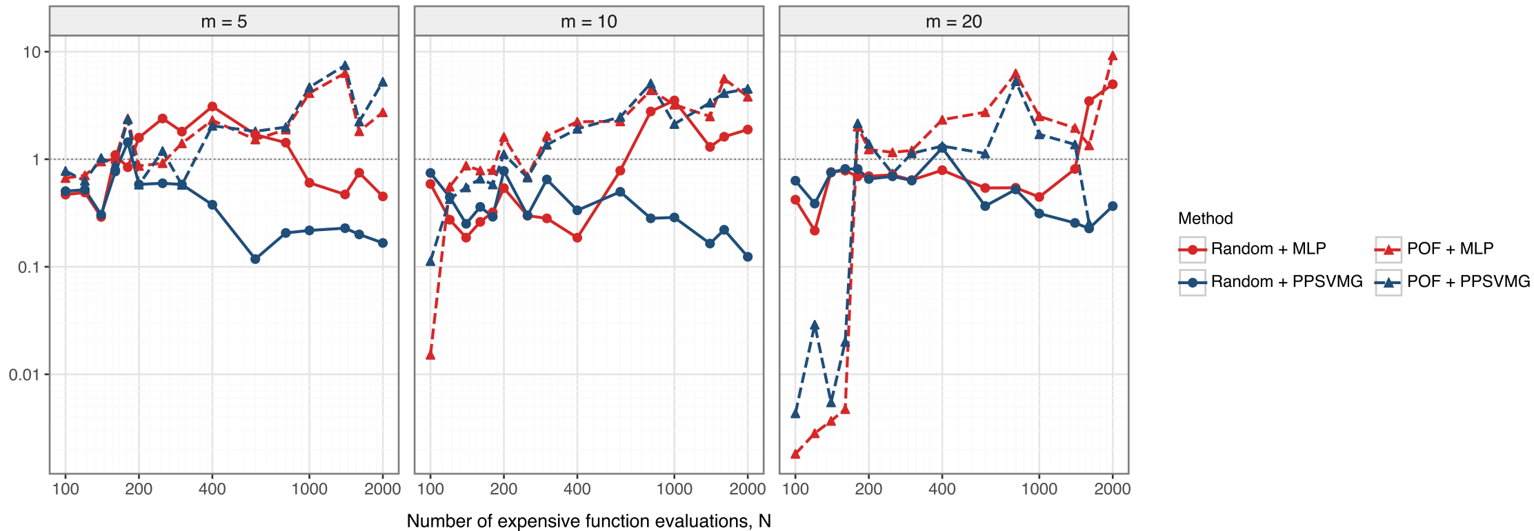
Variance ratio relative to two-stage Monte Carlo
