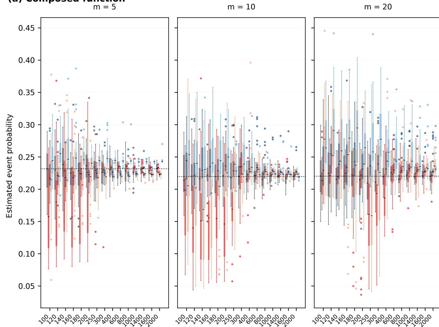
(a) Composed function
