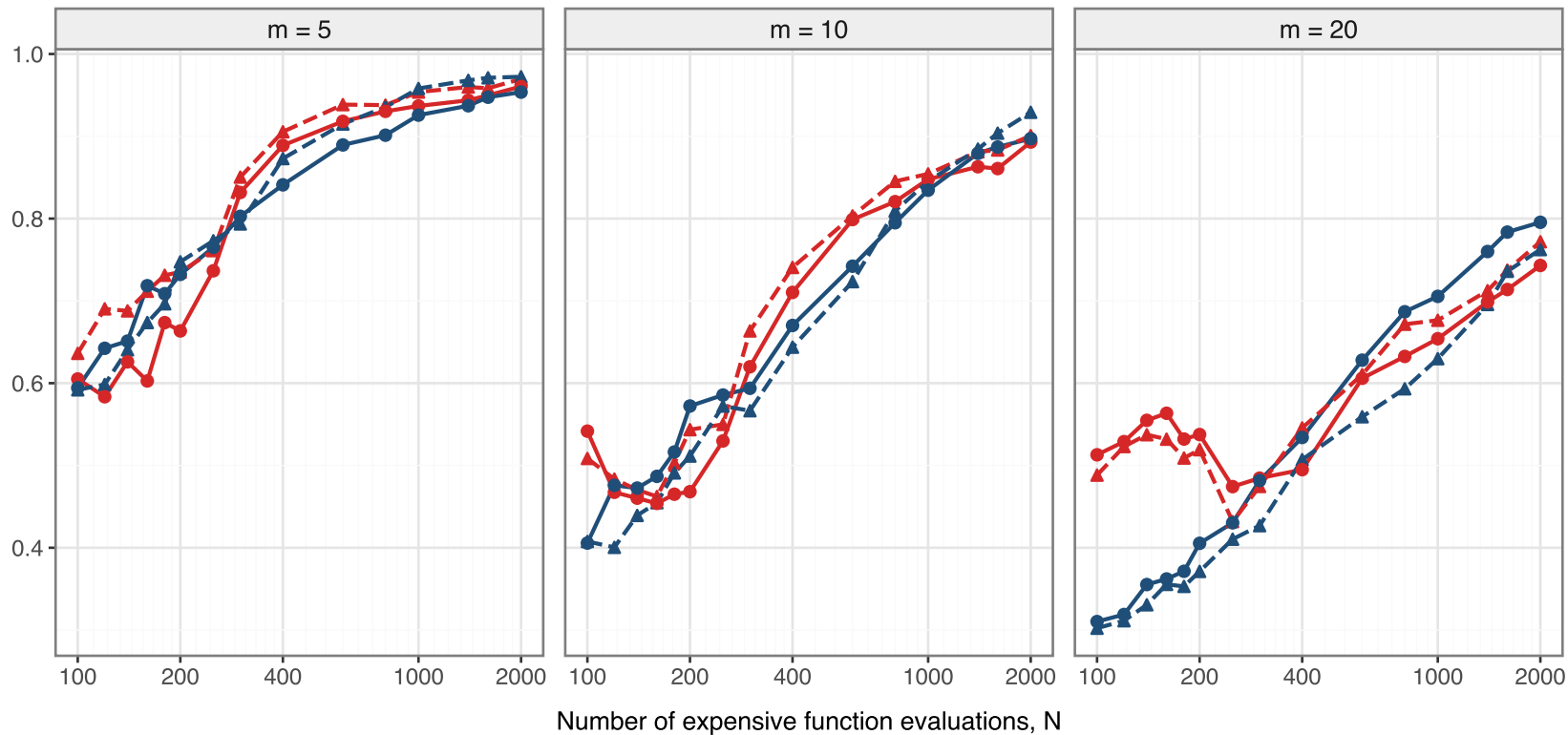
Mean classifier accuracy on 5000-point test set
