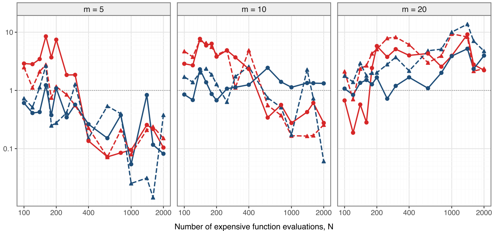
Variance ratio relative to two-stage Monte Carlo
