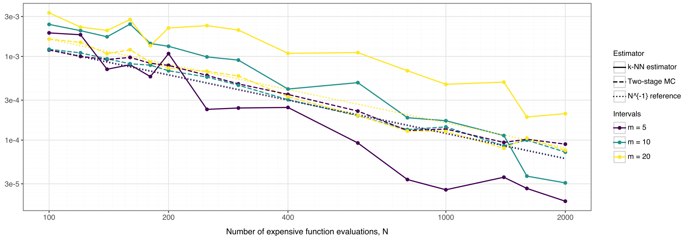
Sample variance of P(E) estimator
