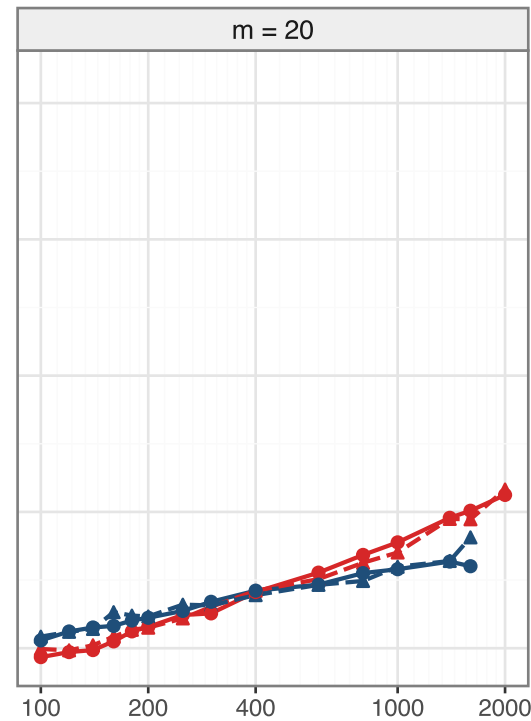
Method
