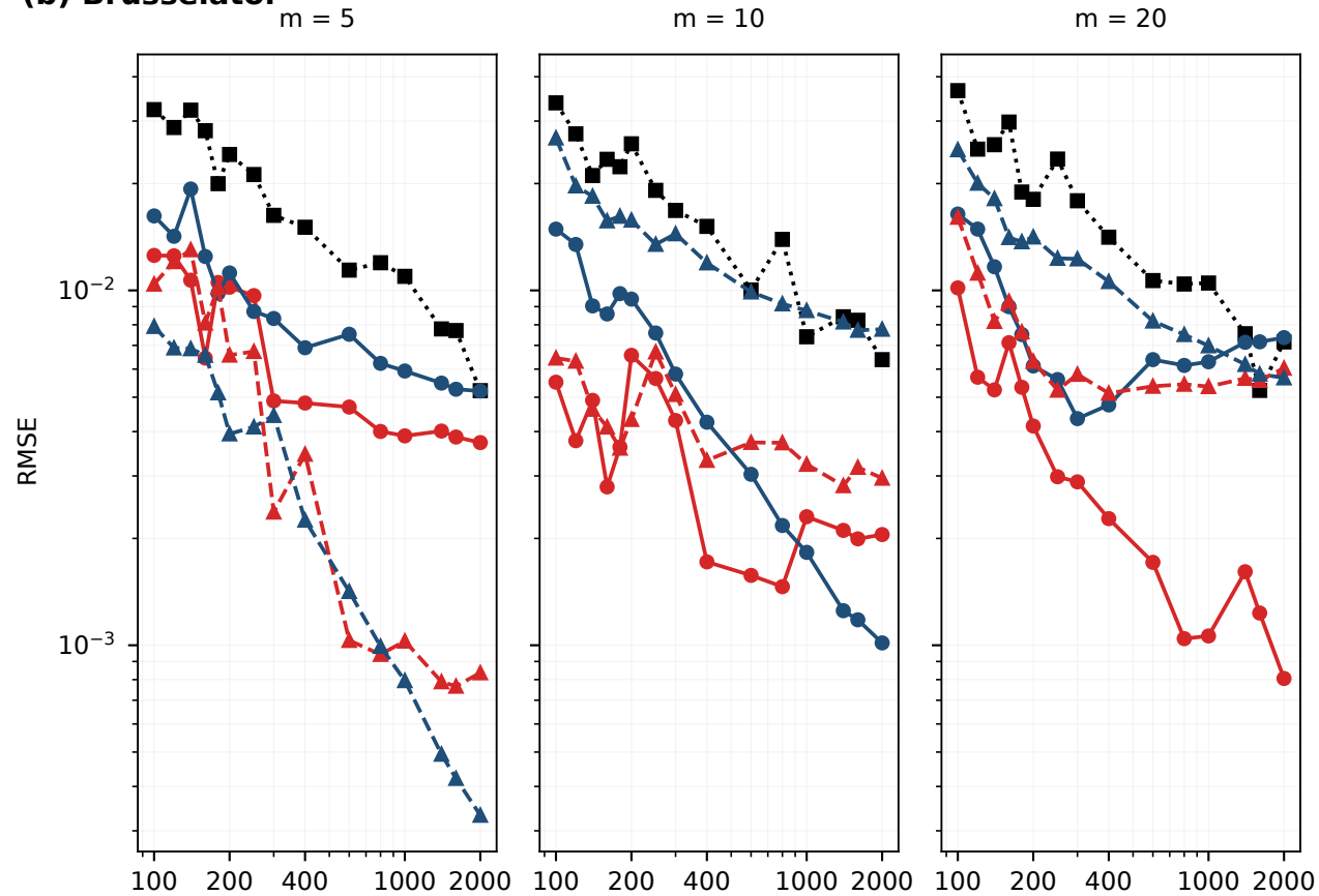
(b) Brusselator
