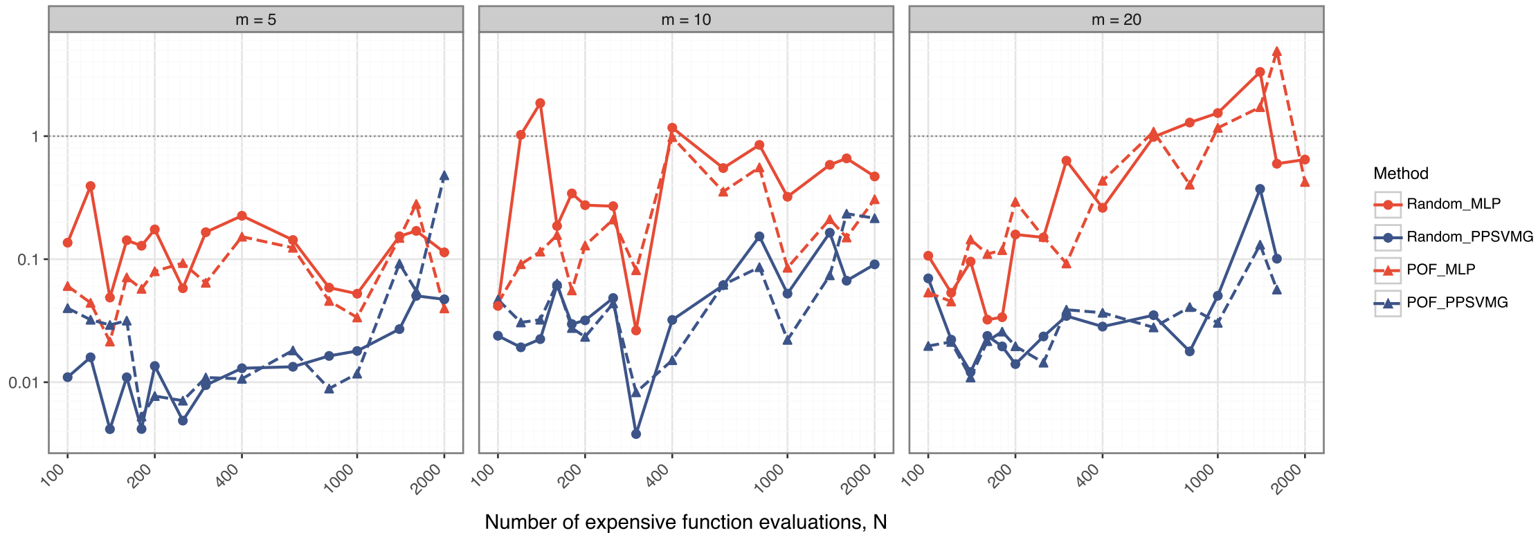
lotka: variance ratio (&lt; 1 = better than naive)
