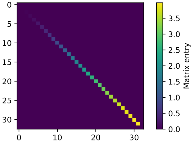
Diagonalized potential O^T VO
