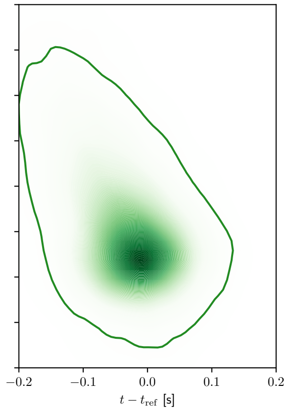
Time at merger
