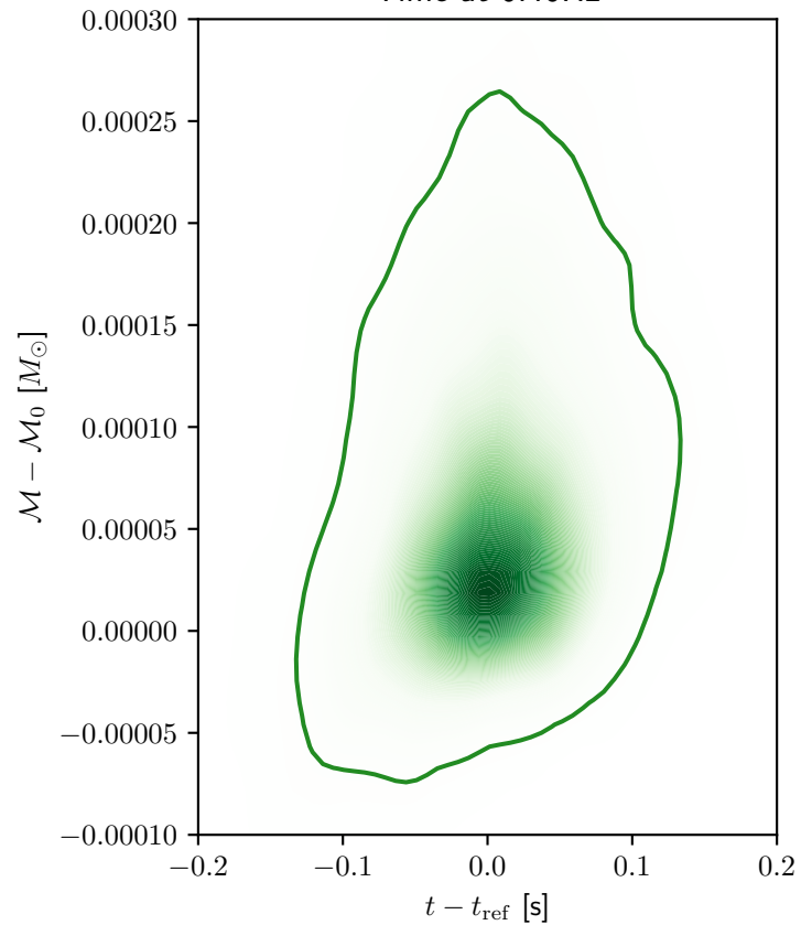
Time at 0.40Hz
