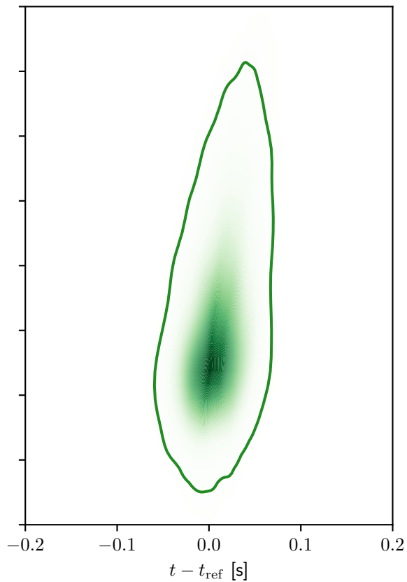
Time at 0.54Hz
