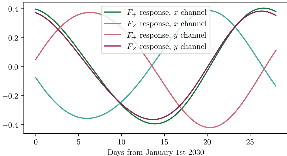
Antenna patterns for a source at declination 90 degrees
