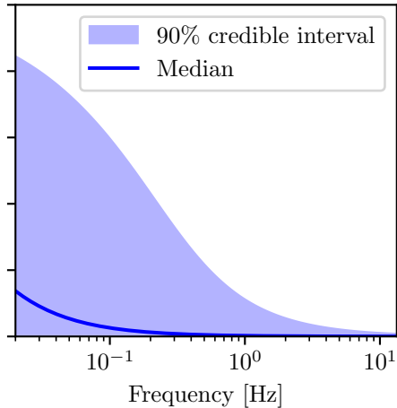
Log-uniform prior on e_{13.33\text{Hz}}
