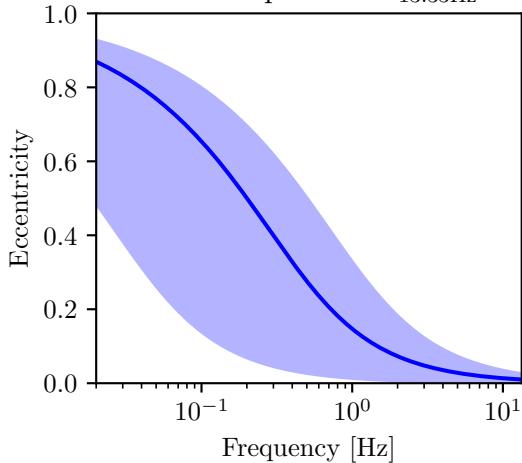
Uniform prior on e_{13.33\text{Hz}}
