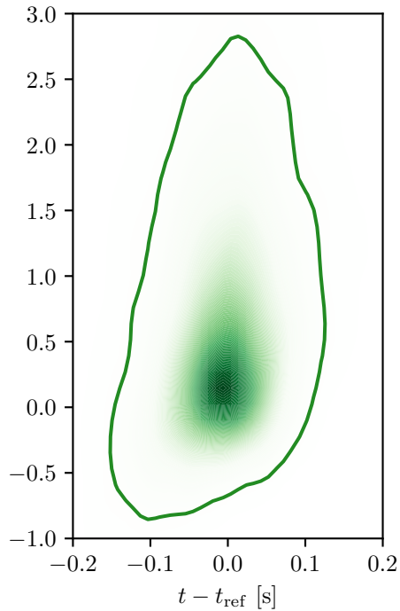
Time at 0.40Hz
