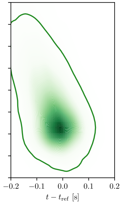
Time at merger
