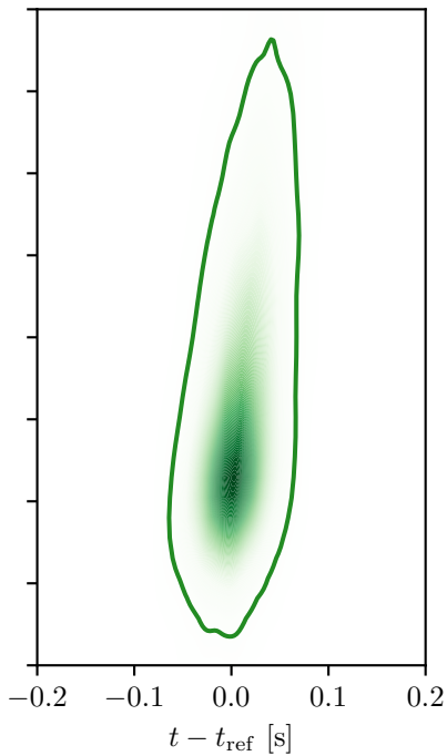
Time at 0.54Hz
