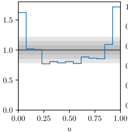
Histogram
