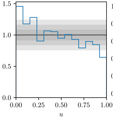
Histogram
