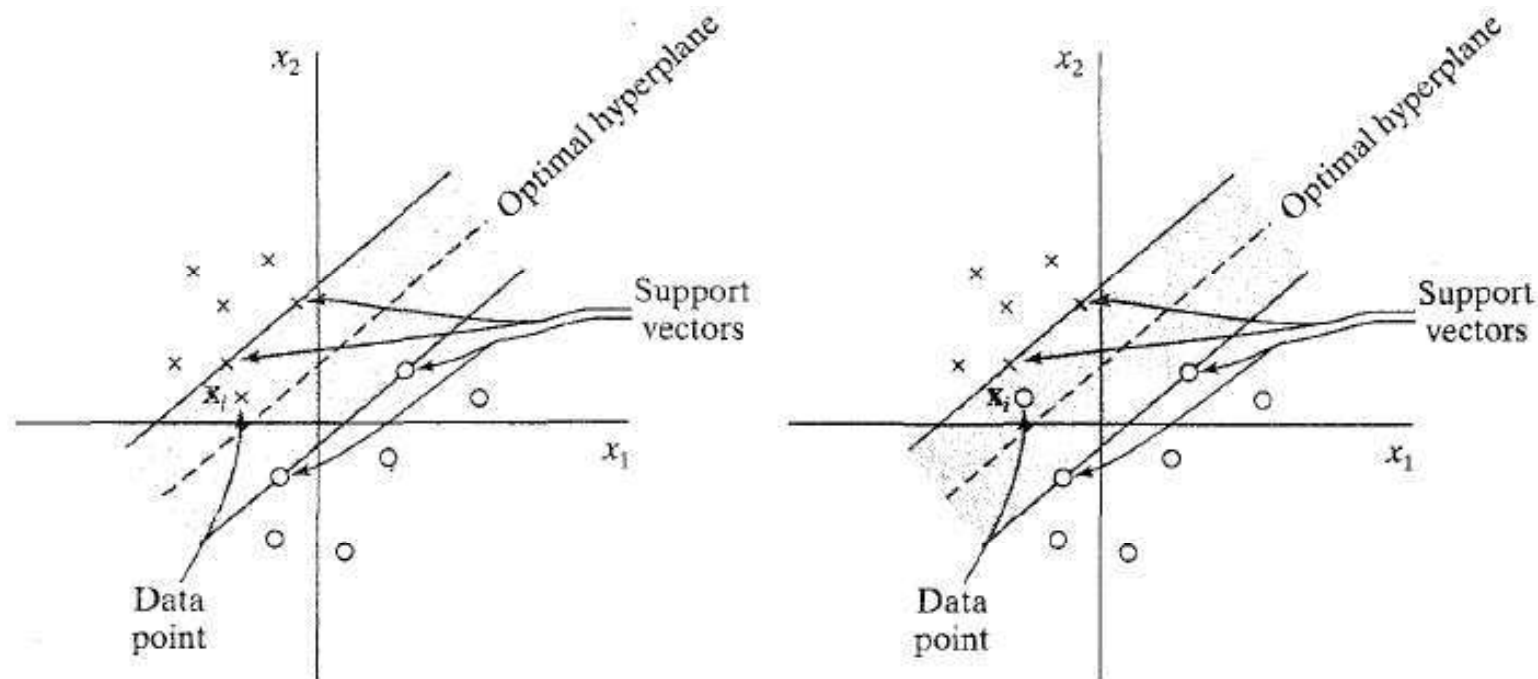
Figure: Patterns violating the margin (with and without classification error).
