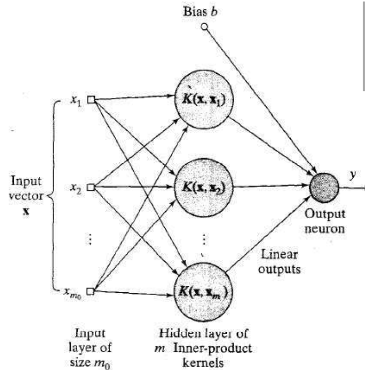
Figure: “Architecture” of a SVM.
