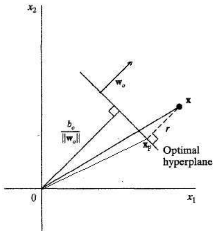
Figure: Distance between a point and the optimum hyperplane.
