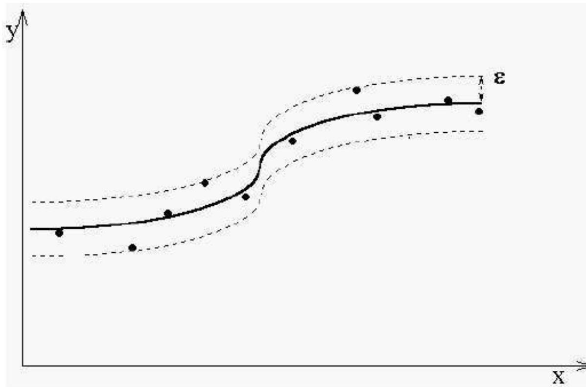
Figure: \epsilon -tube around d .
