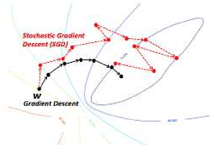
Stochastic Gradient Descent
