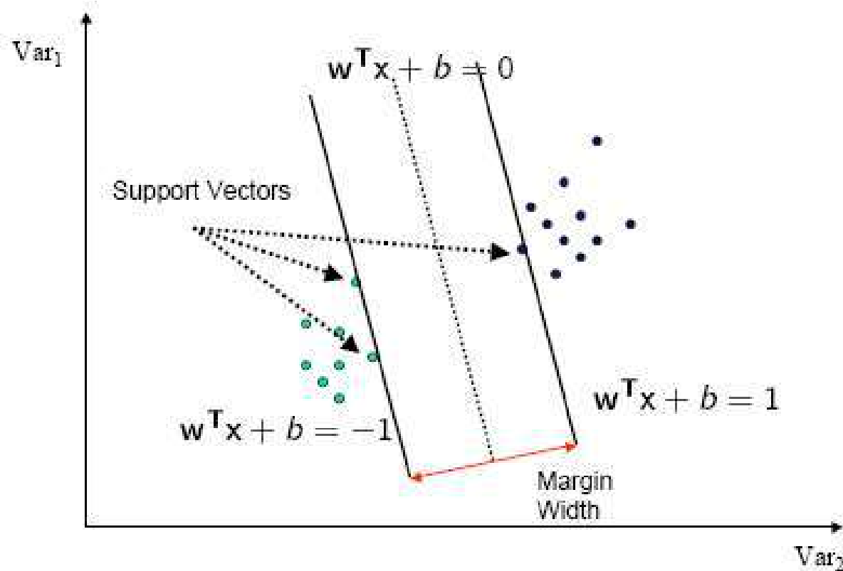
Figure: Support vectors.
