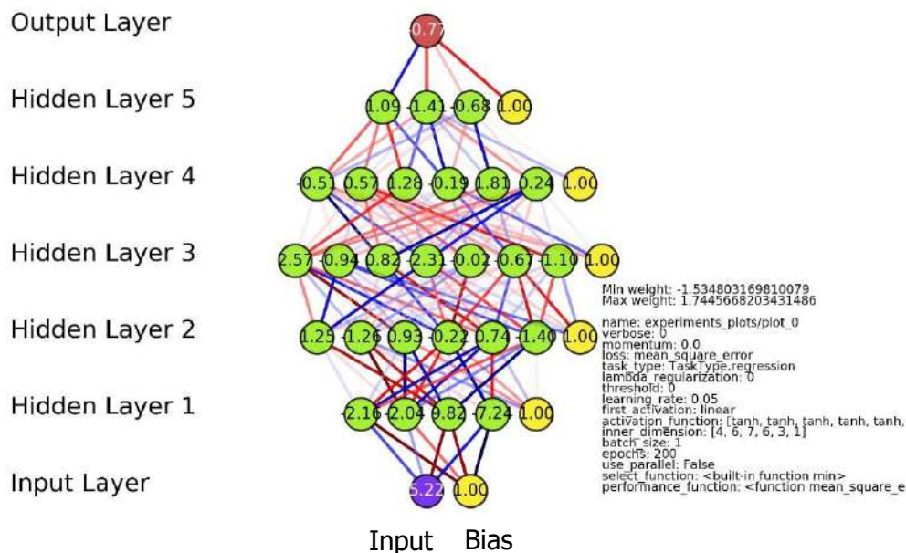
Neural Network architecture
