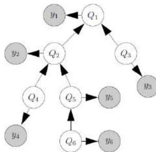
Bottom-up Hidden Tree Markov Models (2012)
