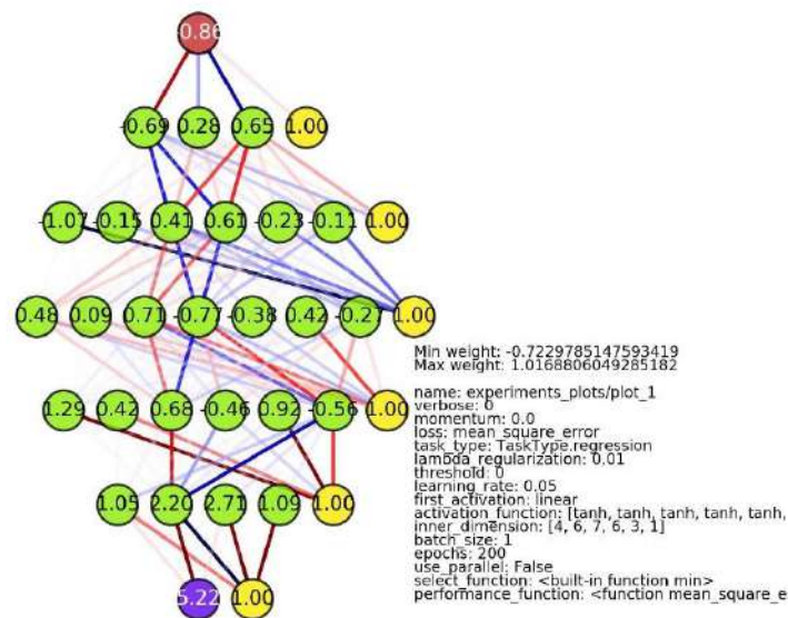
Neural Network architecture
