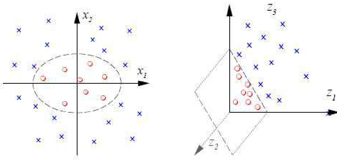
Figure: In the input space we need a quite complex decision surface, while in the second order monomials feature space a linear function is sufficient.
