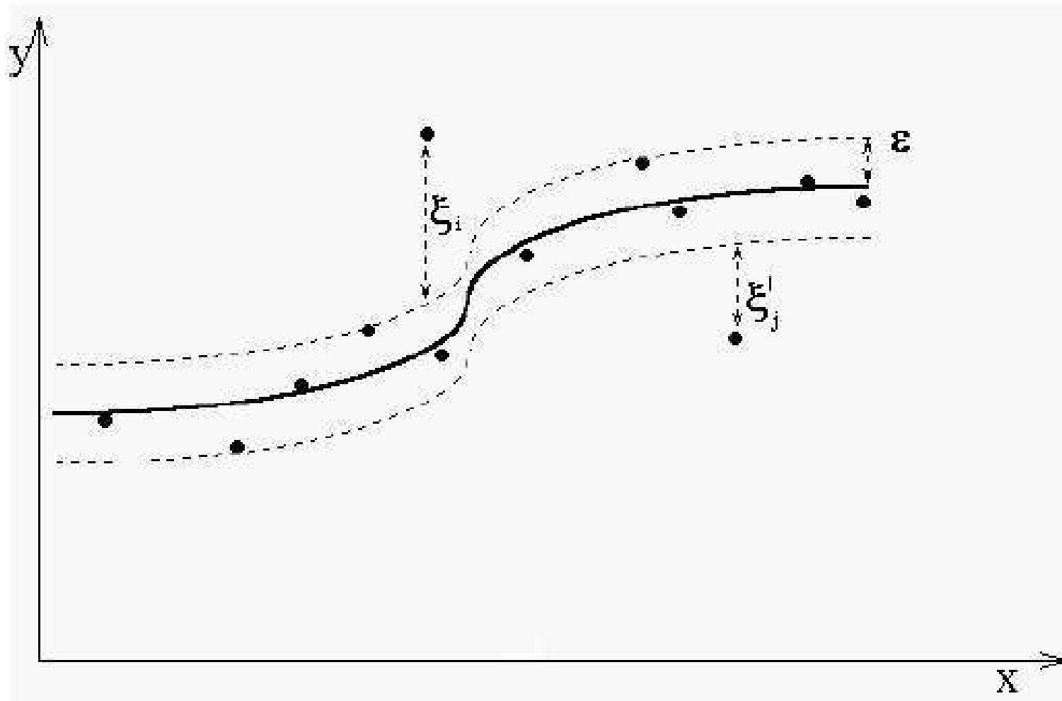
Figure: \epsilon -tube and slack variables.
