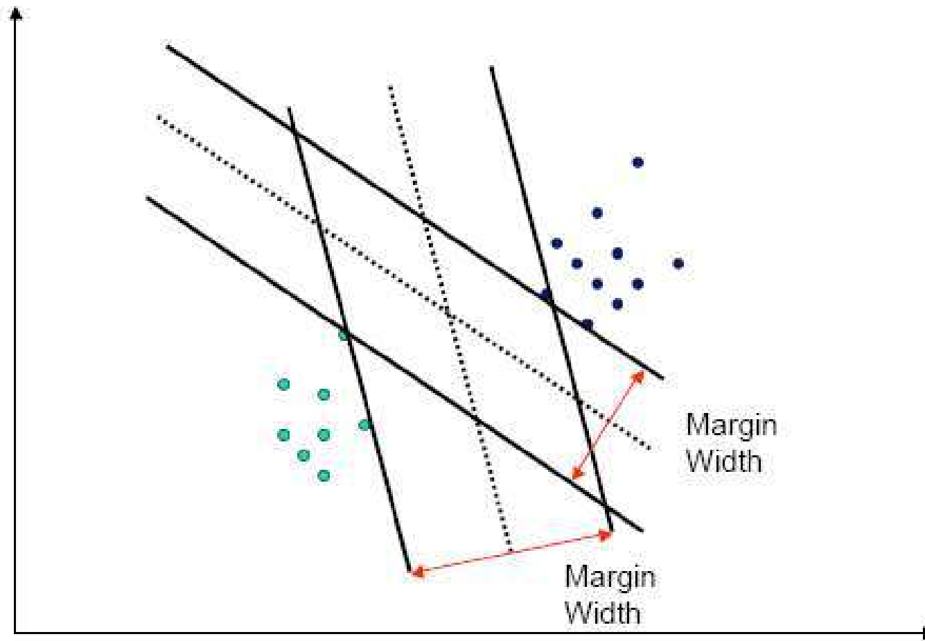
Figure: Varying the separating hyperplane the margin varies as well.
