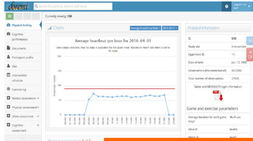
Web-based Dashboard
