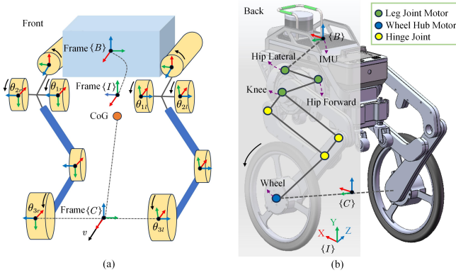
Fig. 2. (a) Kinematic model and coordinate system definition of the WBR. (b) Mechanical structure and motor distribution of the WBR. The robot has eight motors in total, with green circles representing the leg motors and blue circles indicating the wheel hub motors. The hip lateral motors allow for the abduction and adduction of the legs. The hip forward and knee motors coordinate to control the pose of the floating base. In this work, the rotation of the hip lateral motors is not considered. \theta_{1l}, \theta_{1r}, \theta_{2l}, \theta_{2r}, \theta_{3l} and \theta_{3r} represent the rotational angles of the hip forward motors, knee motors, and wheel hub motors, respectively, which are directly measured by encoders. The euler parameters of the floating base are measured by the built-in inertial measurement unit (IMU).
