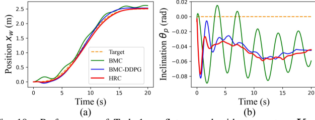
Fig. 10. Performance of Task 1 on flat ground with parameters K_1 . (a) Position x_w change curve. (b) Inclination angle \theta_p change curve.
