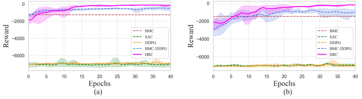
Fig. 3. Comparison of the mean reward between the BMC, SAC, DDPG, BMC-DDPG and HRC during training process. (a) Group 1. (b) Group 2.
