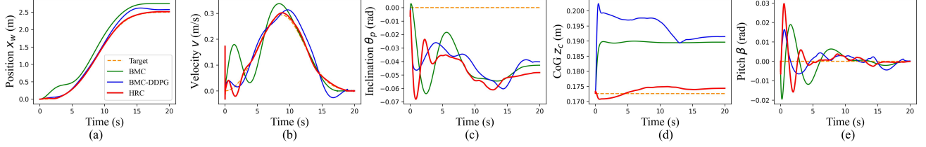
Fig. 4. Performance of Task 1 on flat ground: (a) Position x_w change curve. (b) Velocity v change curve. (c) Inclination angle \theta_p change curve. (d) CoG height z_c change curve. (e) Pitch angle \beta change curve.
