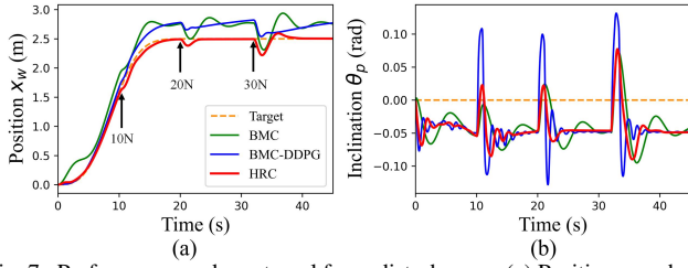
Fig. 7. Performance under external force disturbances. (a) Position x_w change curve. (b) Inclination angle \theta_p change curve.
