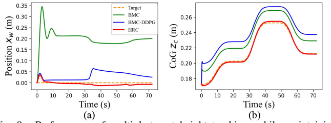
Fig. 9. Performance of multiple-target height tracking, while maintaining position stable. (a) Position x_w change curve. (b) CoG height z_c change curve.
