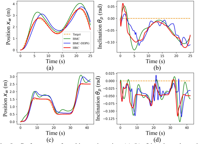
Fig. 8. Performance of tracking trajectories. (a)-(b): 5th-order polynomial random point fitting trajectory. (c)-(d): High-dynamic multi-target trajectory.
