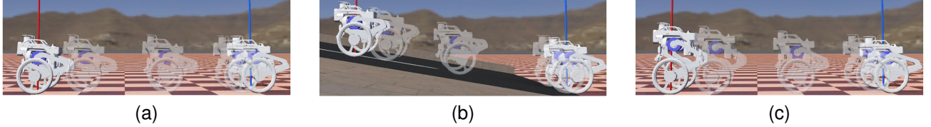
Fig. 6. Task demonstration. (a) Task 1 on flat ground. (b) Task 1 on slope with 10 deg. (c) Task 2 on flat ground.
