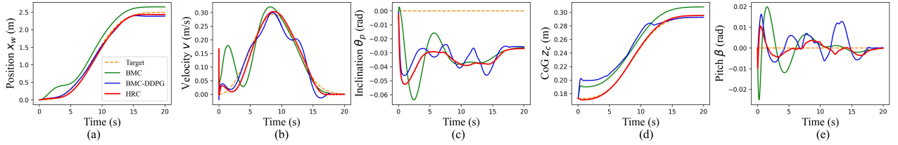
Fig. 5. Performance of Task 2 on flat ground: (a) Position x_w change curve. (b) Velocity v change curve. (c) Inclination angle \theta_p change curve. (d) CoG height z_c change curve. (e) Pitch angle \beta change curve.
