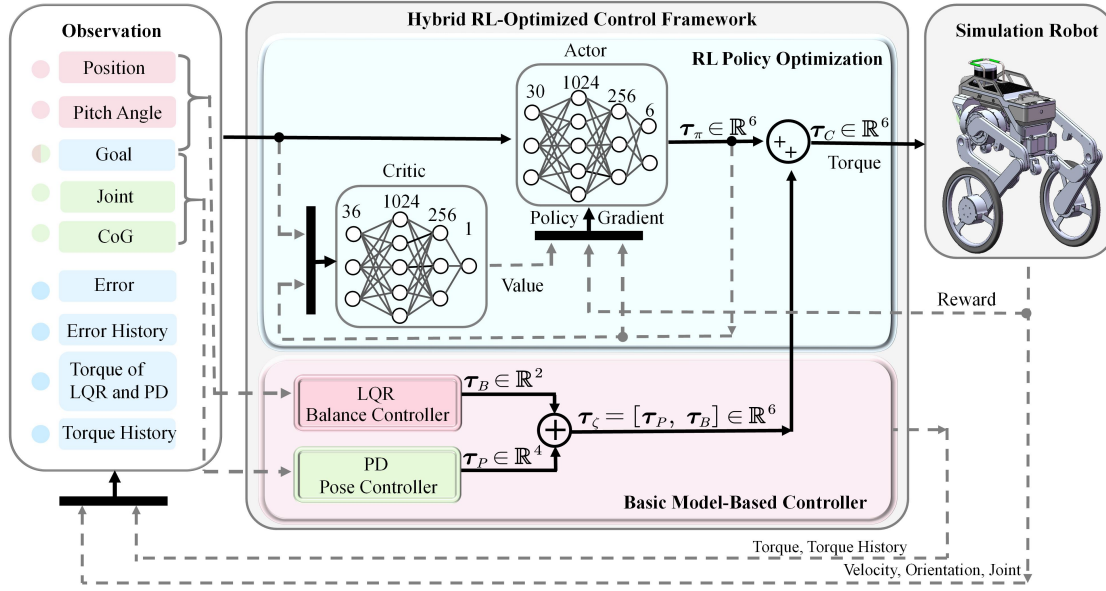
Fig. 1. The hybrid RL control training framework of the WBR. It consists of two modules: the basic model-based controller that ensures system stability, and the RL policy that optimizes control performance in real-time. Both directly generate control torques, which are subsequently summed and applied to the robot joint motors, as shown by the solid lines in the diagram.
