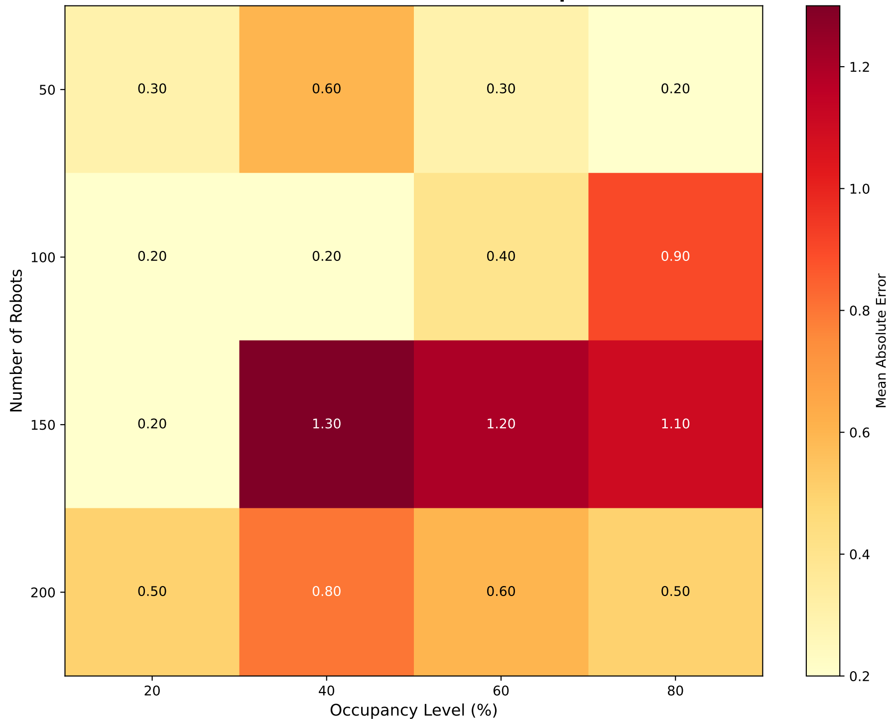
Mean Absolute Error Heatmap
