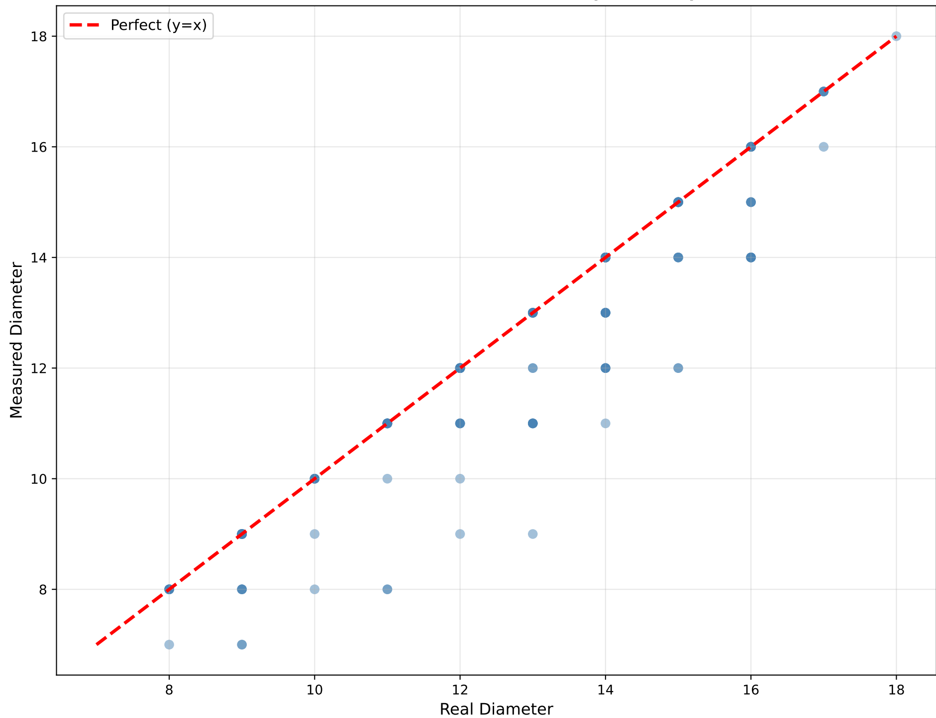
Measured vs Real Diameter (All Trials)
