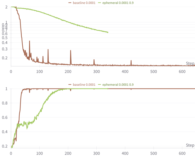
Fig. 5. Performance on the Repeated Sequences task. The baseline, traditional RNN with backprop is used as a benchmark, converging quickly on the loss values and accuracy. Ephemeral weights converge more slowly, but do so without any recurrent connection.
