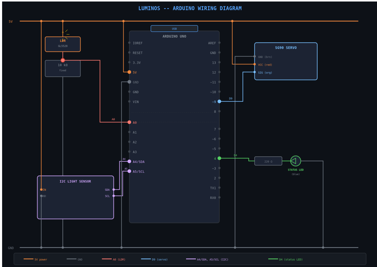
Figure 1: Arduino Uno wiring diagram. Left column (bottom to top): A5/SCL, A4/SDA, A3–A0, VIN, GND (x2), 5V, 3.3V, RESET, IOREF. Right column (top to bottom): AREF, GND, 13–8, 7–0. Highlighted pins are those used in this prototype.
