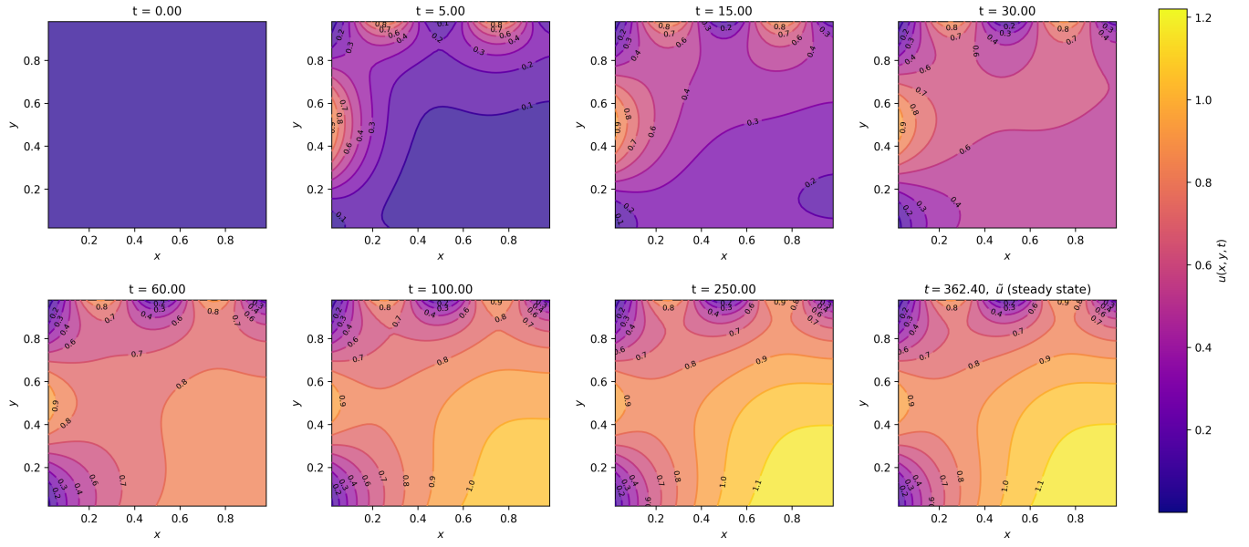
FIG. 3 Transient solution u(x, y, t) at selected timesteps, marching from u(x, y, 0) = 0 to steady state using Crank–Nicolson time integration.
