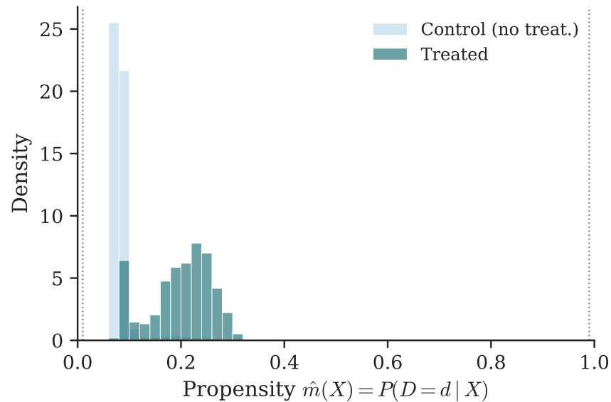
Boil (trimmed 0.0%)
