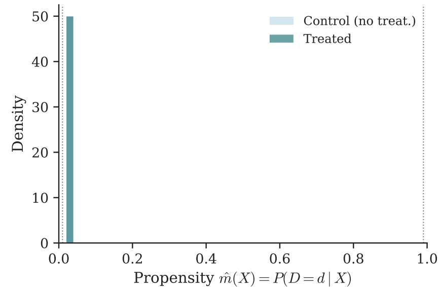
Chlorine (trimmed 0.0%)
