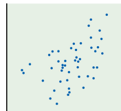
Correlation r = 0.5
