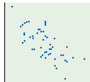
Correlation r = -0.7
