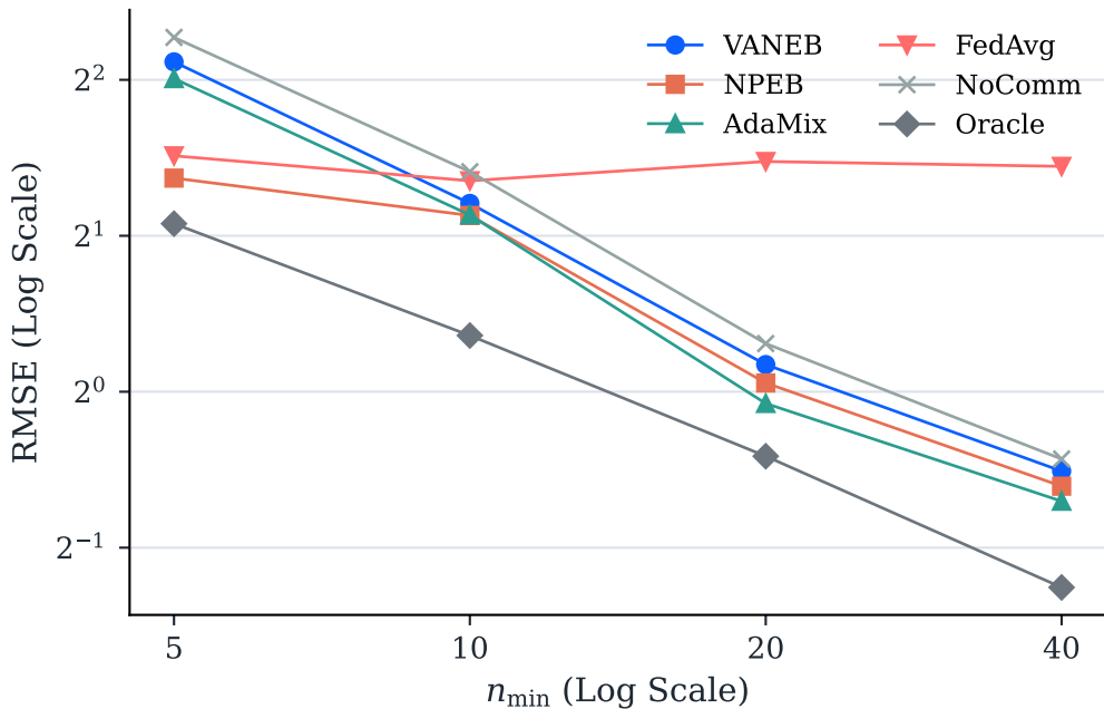
Multiclass logistic (Log-Log)
