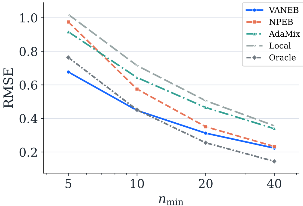
Quadratic variance (Log x)
