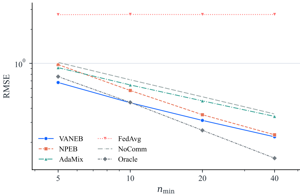
Quadratic variance (Log-Log)
