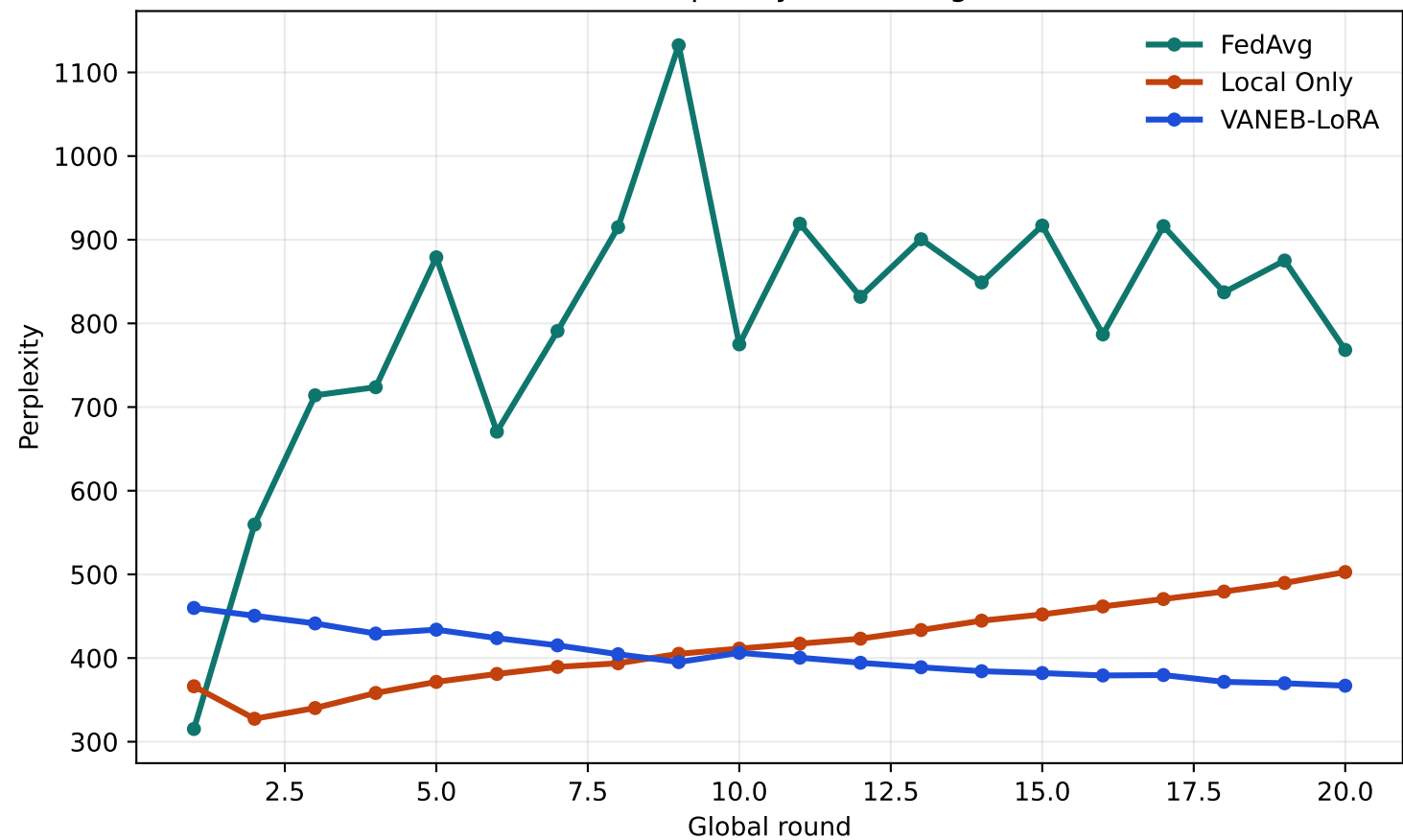
Global Test Perplexity vs Training Round
