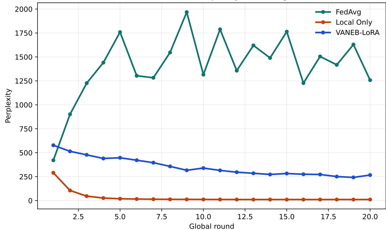
Personalized Holdout Perplexity vs Training Round
