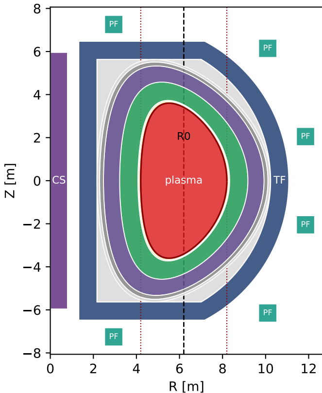
Radial build
