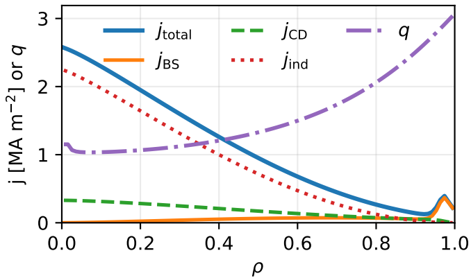
Current density and safety factor
