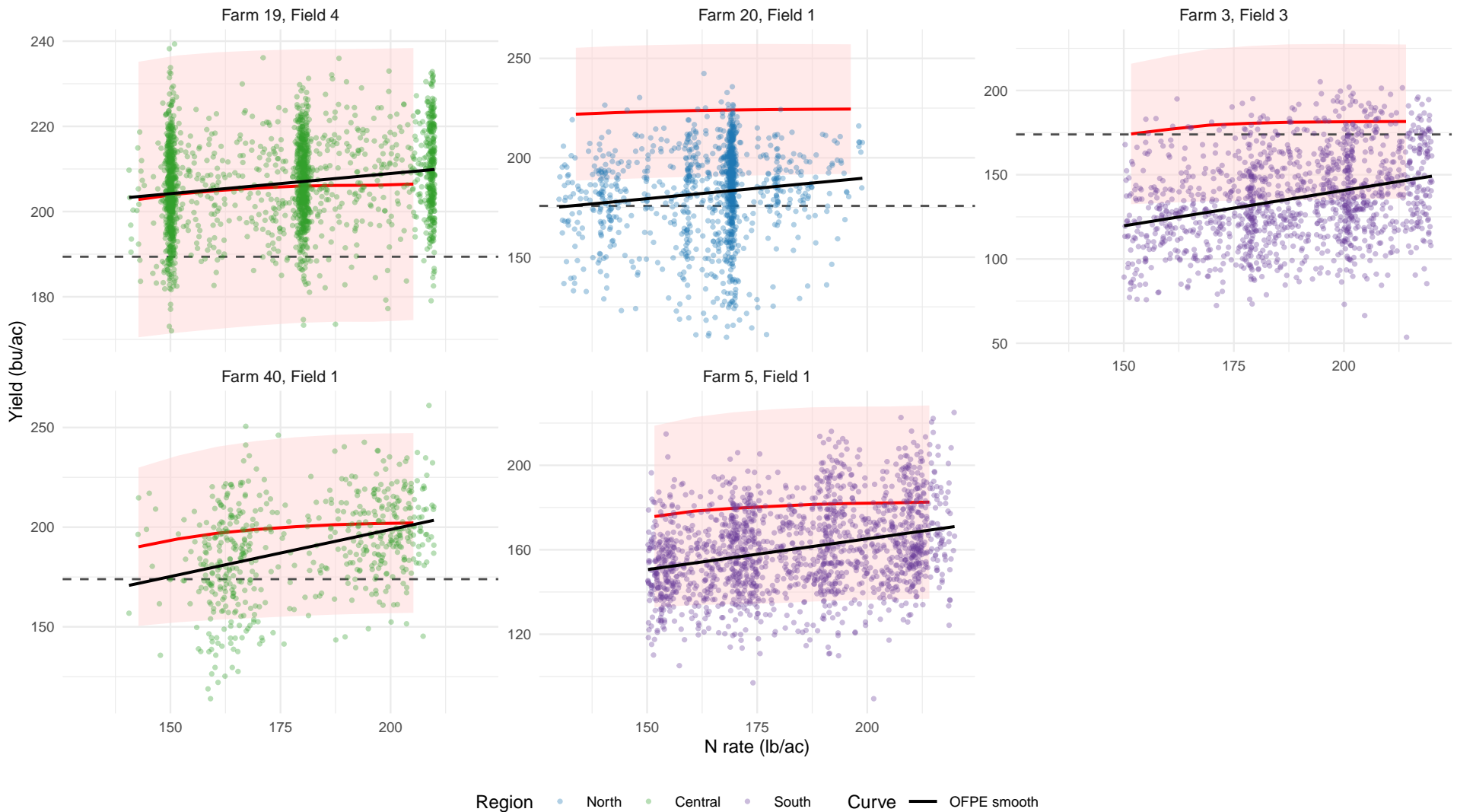
APSIM prior (red, band = mean \pm 1.28 sd) vs OFPE (points, black smooth), year 2019
