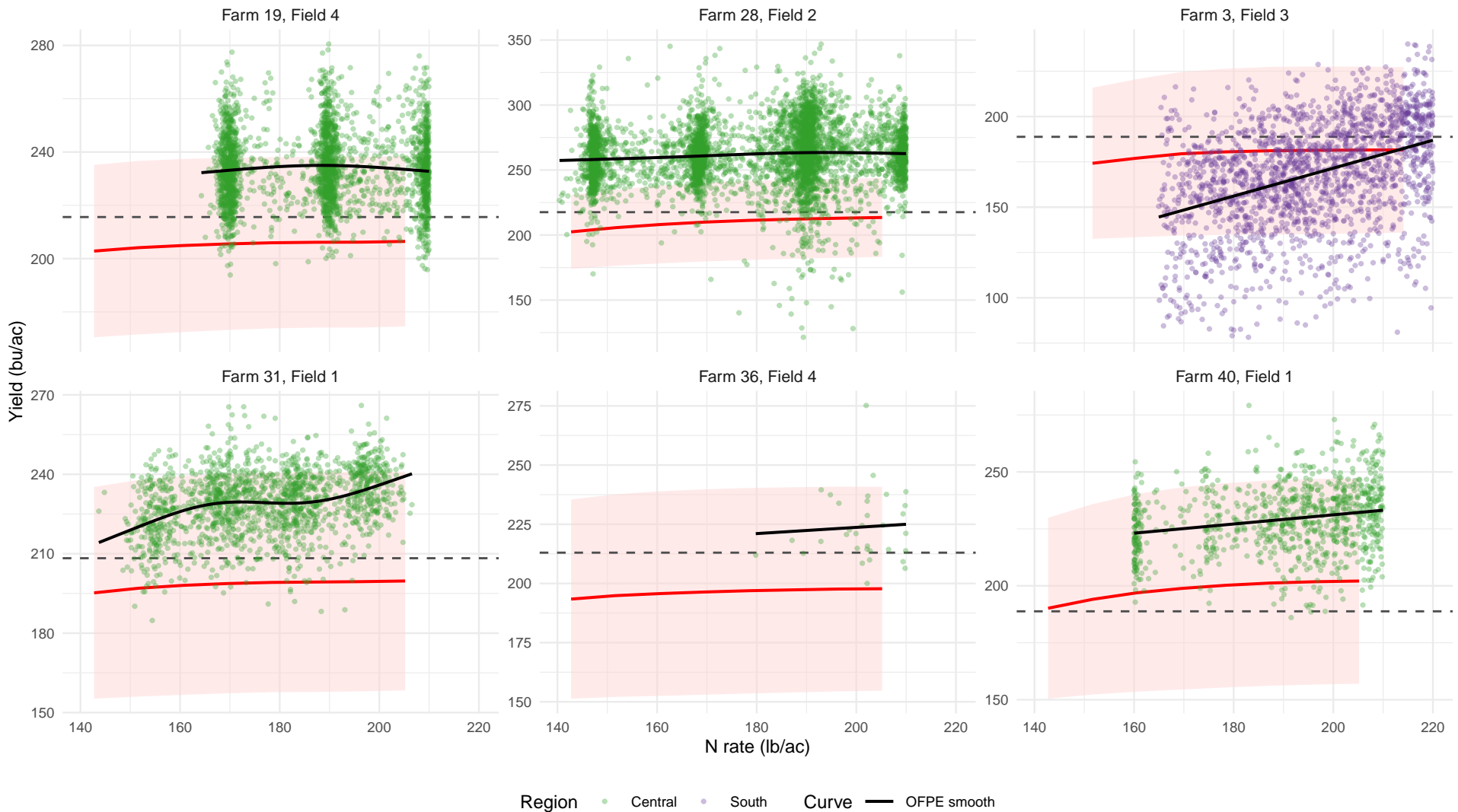
APSIM prior (red, band = mean \pm 1.28 sd) vs OFPE (points, black smooth), year 2017
