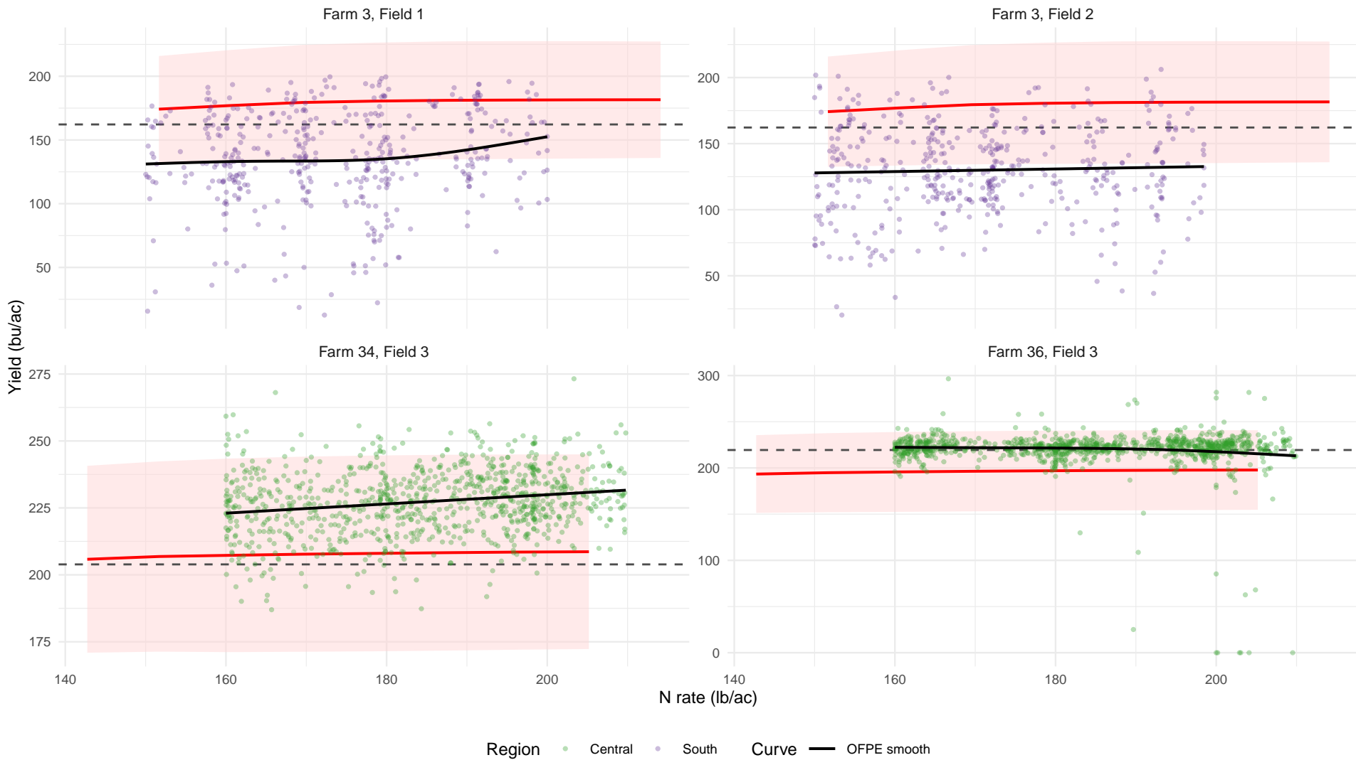
APSIM prior (red, band = mean \pm 1.28 sd) vs OFPE (points, black smooth), year 2016
