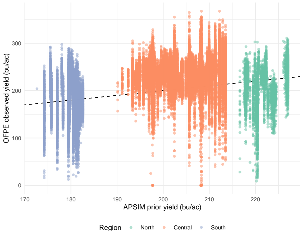
Matched APSIM vs OFPE yields (nearest N per field-year)
