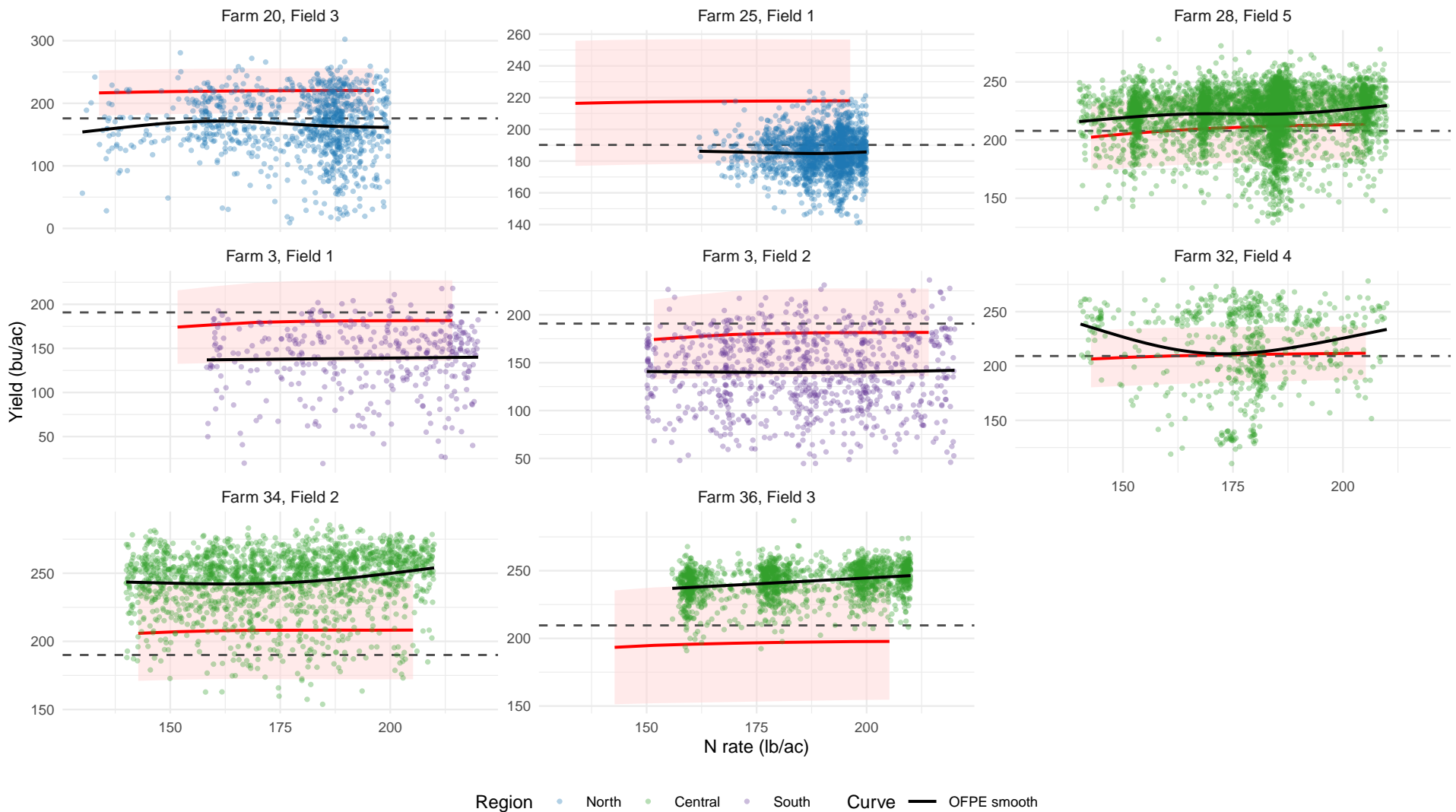
APSIM prior (red, band = mean \pm 1.28 sd) vs OFPE (points, black smooth), year 2020
