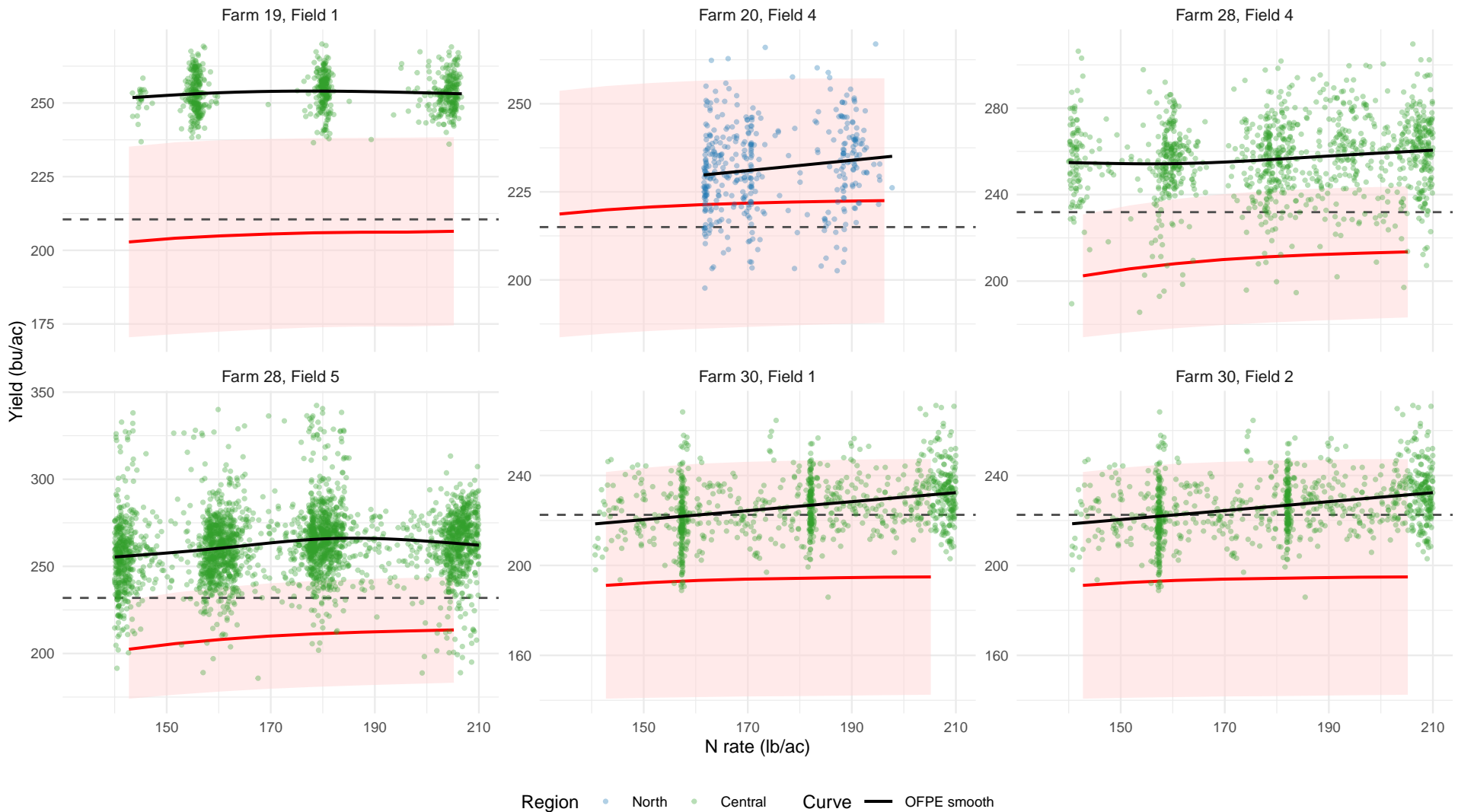
APSIM prior (red, band = mean \pm 1.28 sd) vs OFPE (points, black smooth), year 2022
