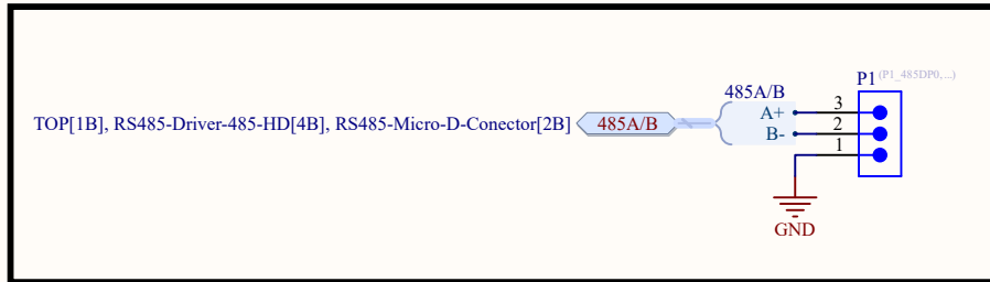
Pin Header Connector for RS485
