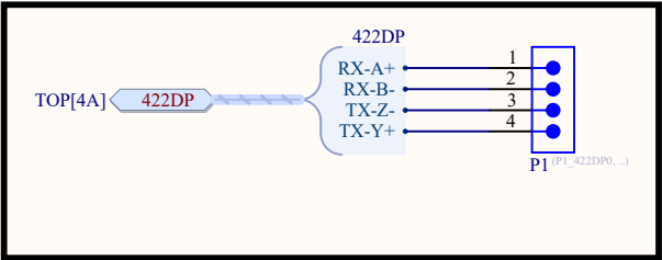
Pin Header Connector for RS422
