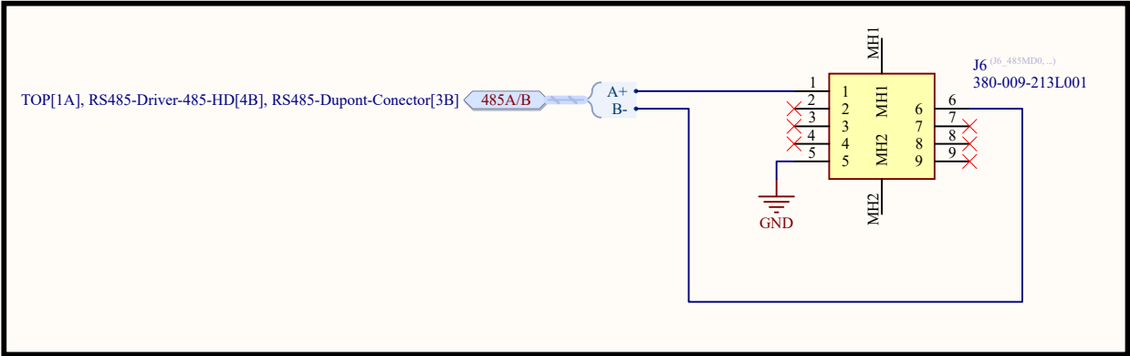
Micro-D Connector for RS485
