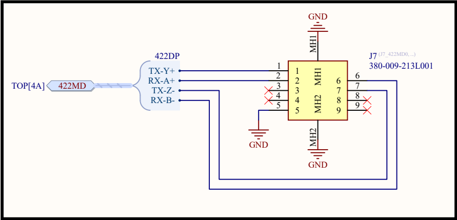
Micro-D Connector for RS422
