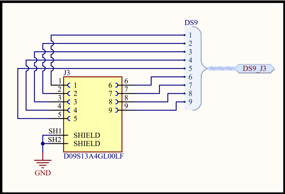
D-Sub 9 Female Conector
