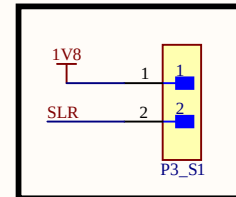
Slew rate control
