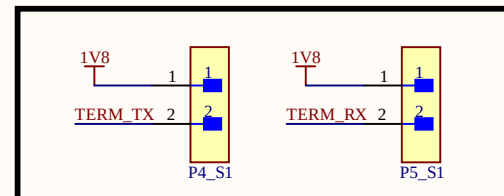
Termination Resistors
