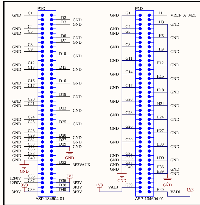
Power and Grounding from FMC Connector
