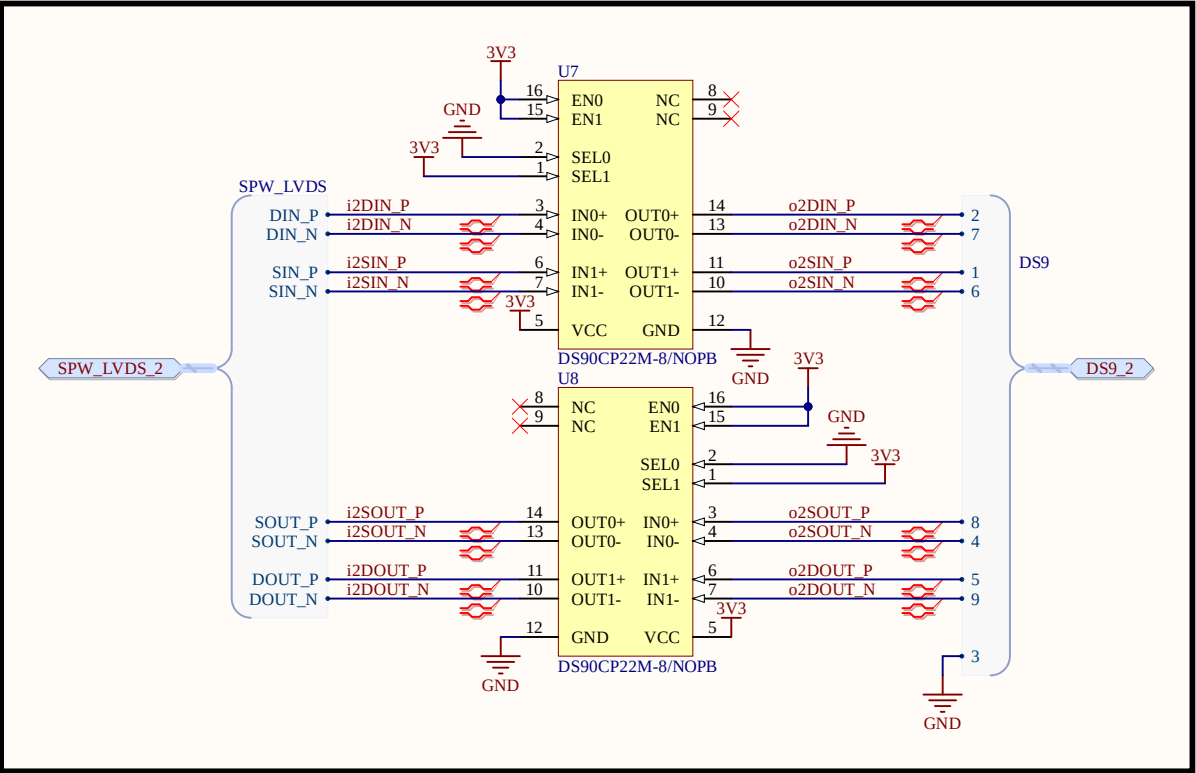
2xLVDS Repeaters, one for transmission and one for reception.
