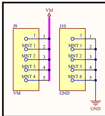
Banana Connectors for Power Supply Power and Ground
