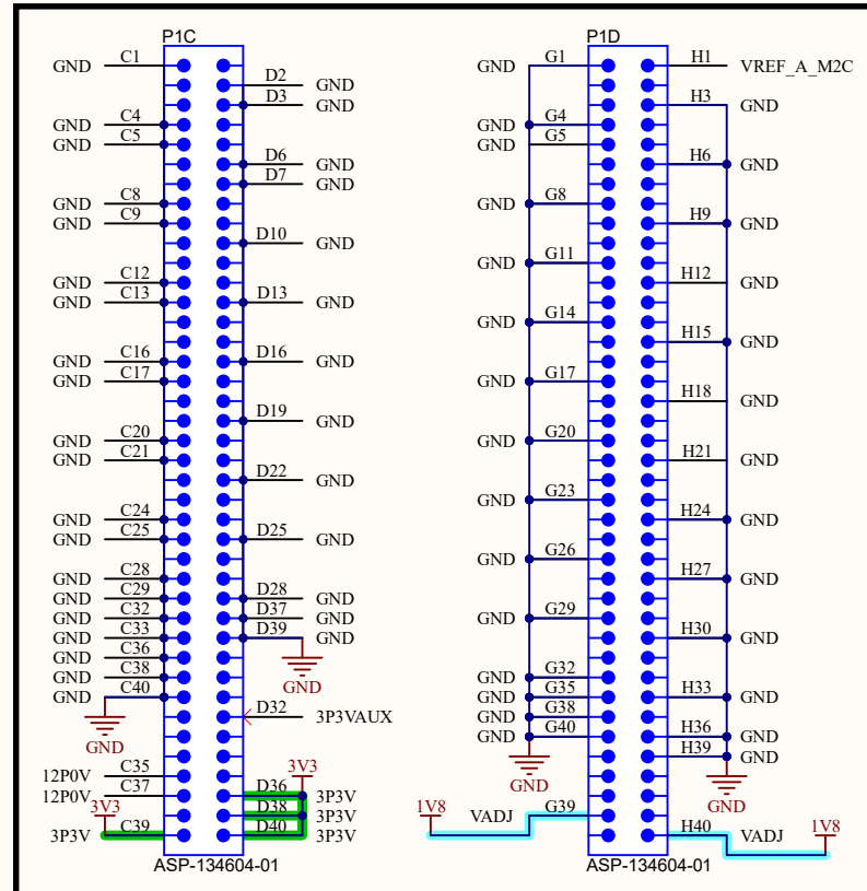
Power and Groung from FMC Conector
