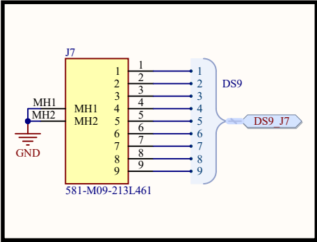
D-Sub 9 Female Conector
