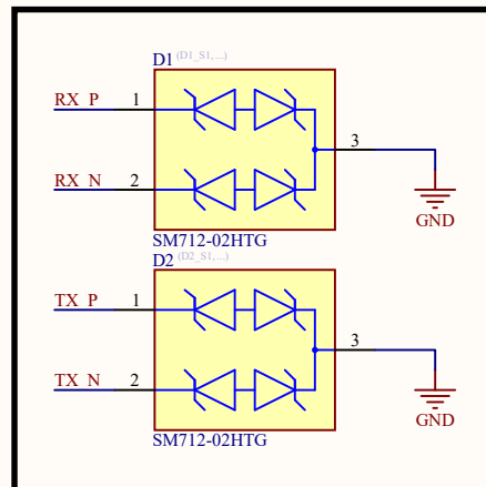
ESD Protection
