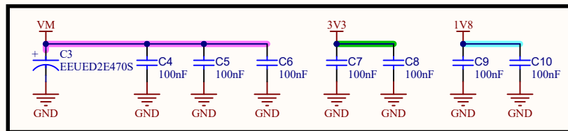
Decoupling Capacitors
