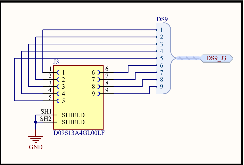
D-Sub 9 Female Conector
