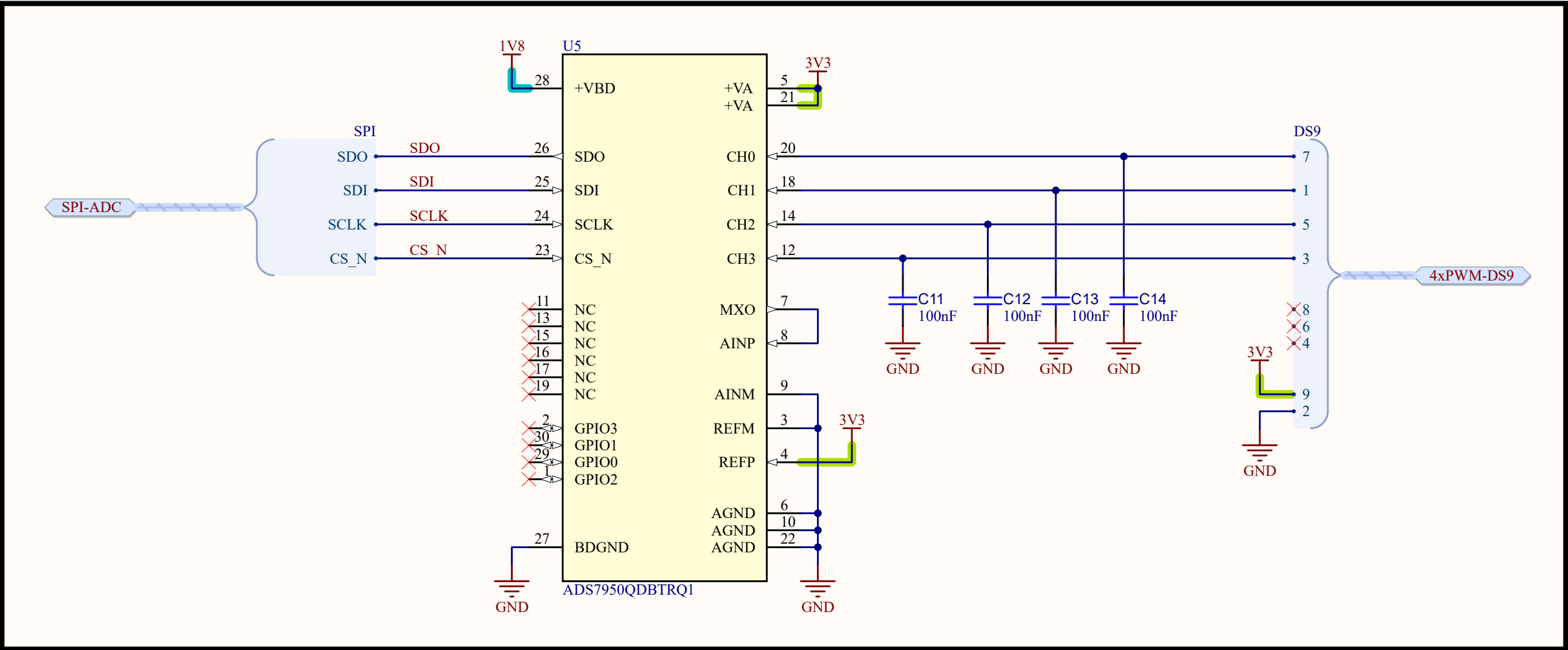
Decoupling Capacitors
