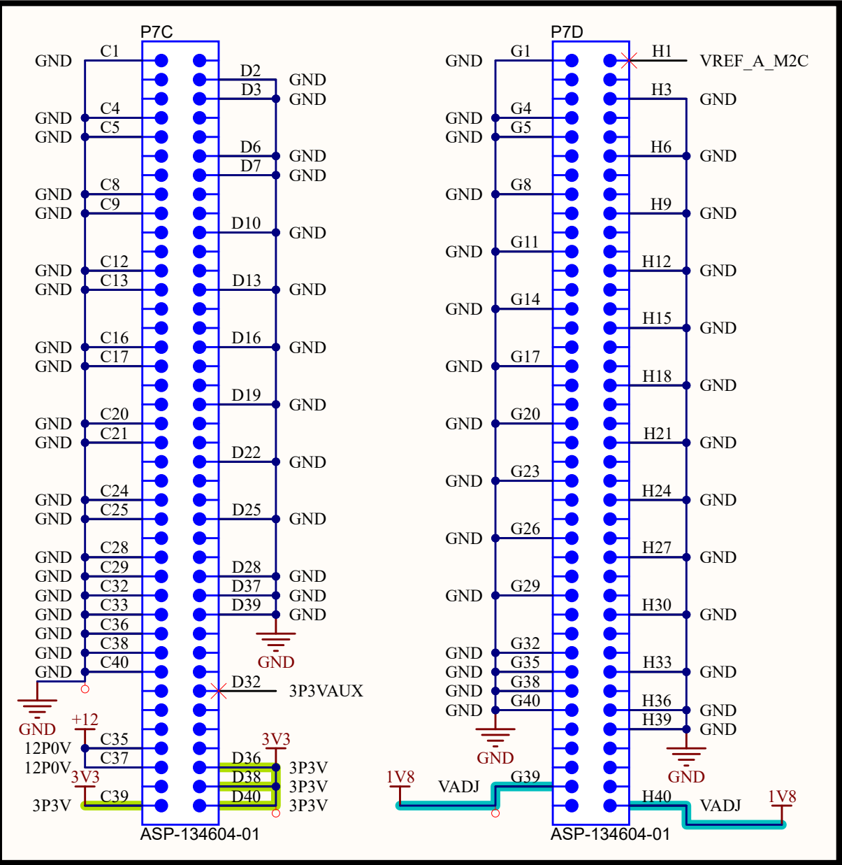
Power and Grounding from FMC Conector
