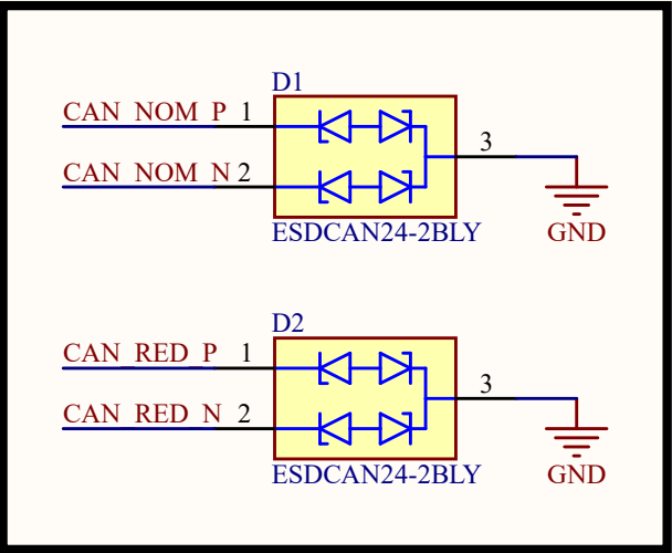
ESD Protection
