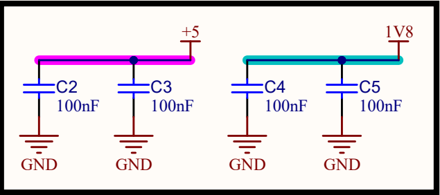
Decoupling Capacitors
