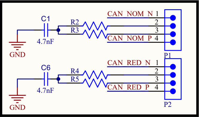
Termination Resistors
