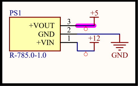
DC/DC Converter
