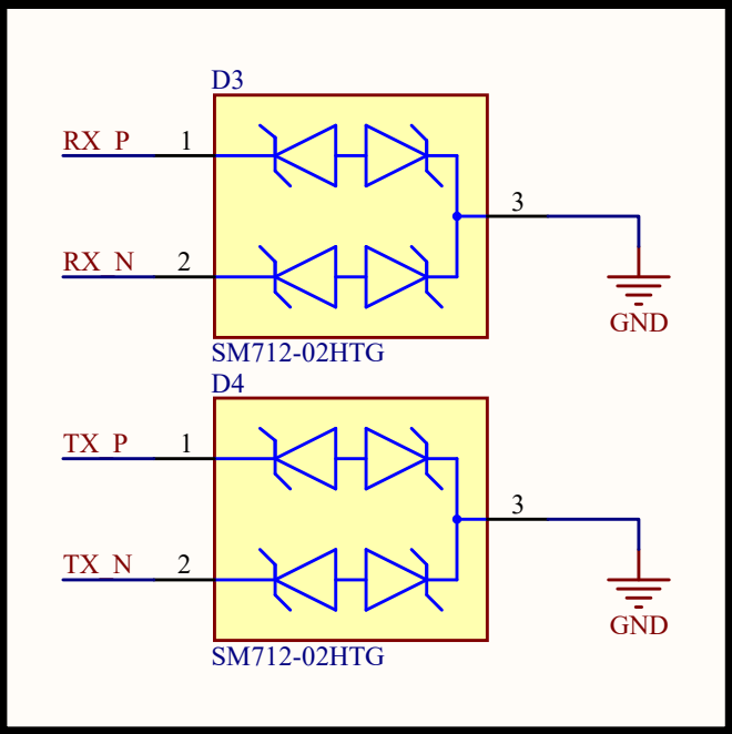
ESD Protection
