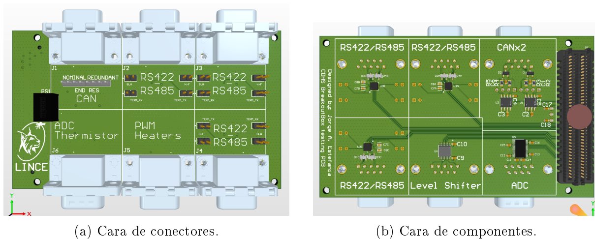
Figura 3.9: Render 3D de la placa CDHS.
