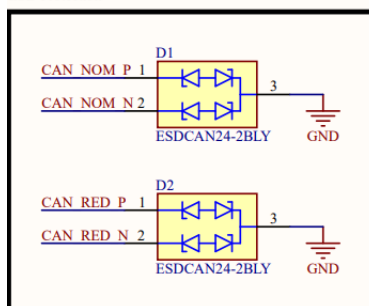
ESD Protection
