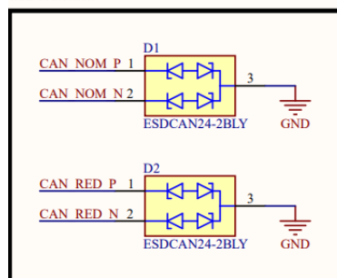
ESD Protection
