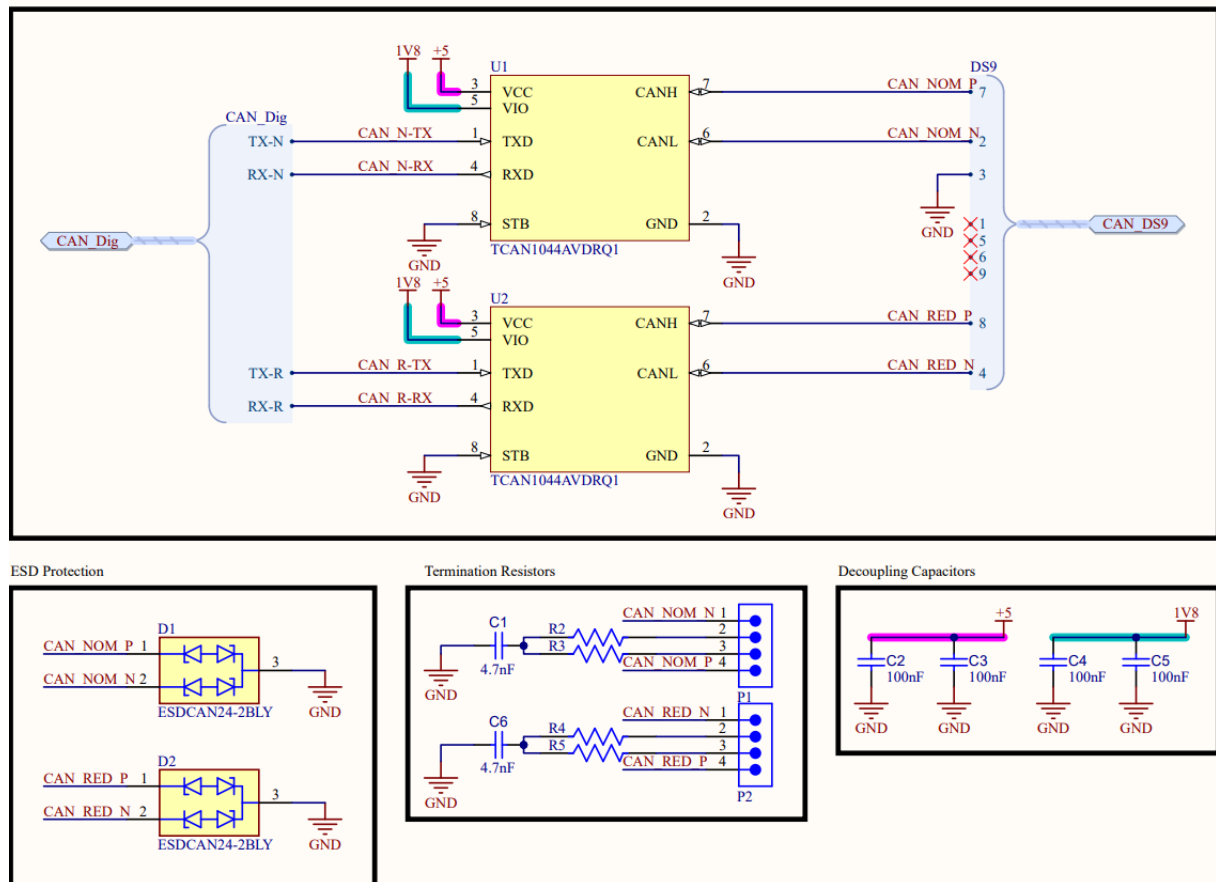
Figura 4.5: Subsistema CAN de la placa CDHS.
