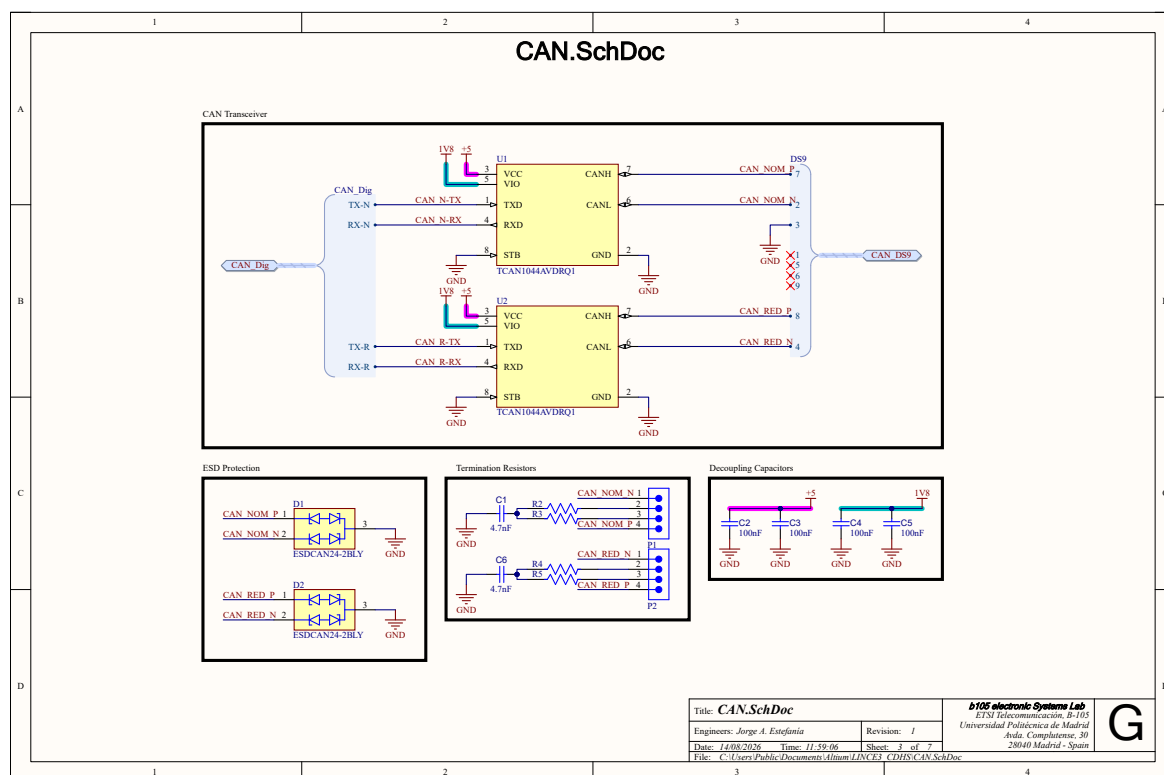
Figura 3.9: Subsistema CAN de la placa CDHS.
