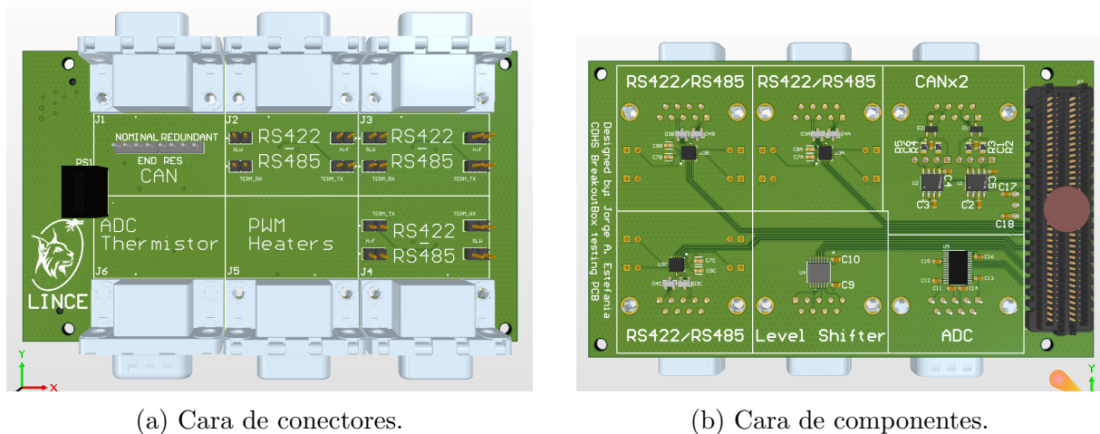
Figura 3.8: Render 3D de la placa CDHS.
