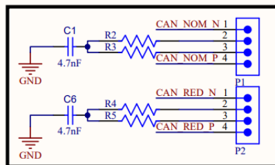
Termination Resistors
