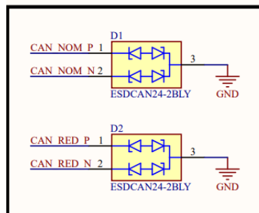
ESD Protection
