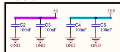
Decoupling Capacitors
