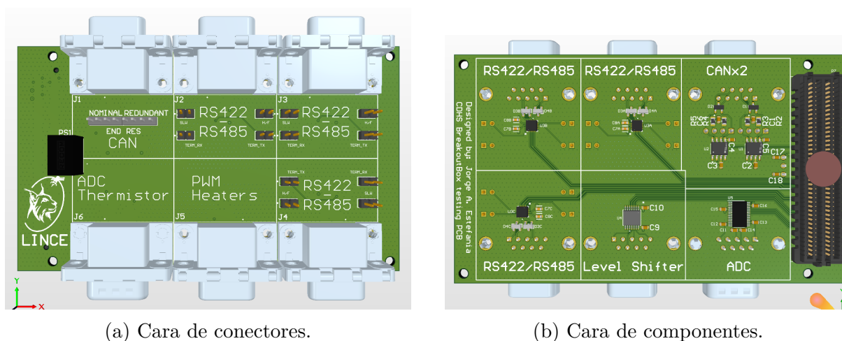
Figura 4.4: Render 3D de la placa CDHS.
