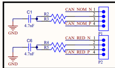
Termination Resistors
