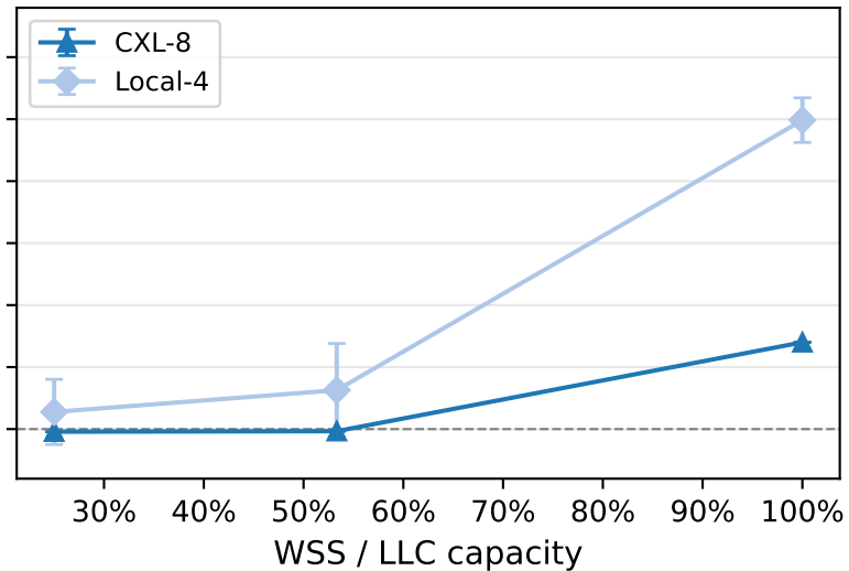
SPR (60 MB LLC)
