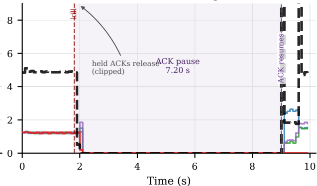
(b) Per-session FIFO hold (prefix-safe)
