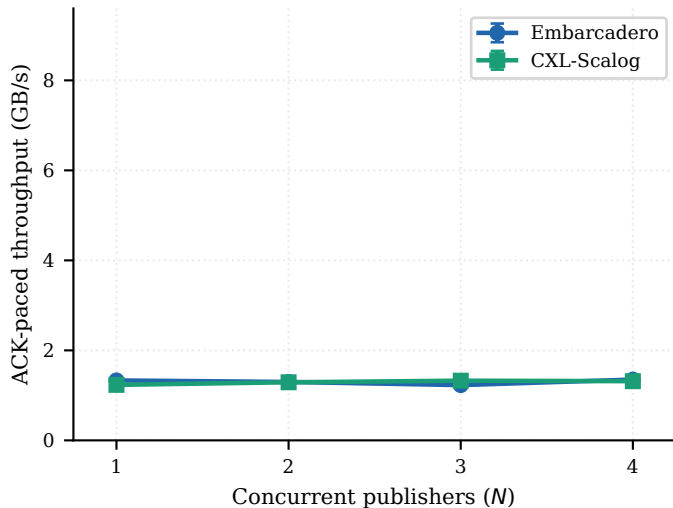
(a) NVMe-durable replica
