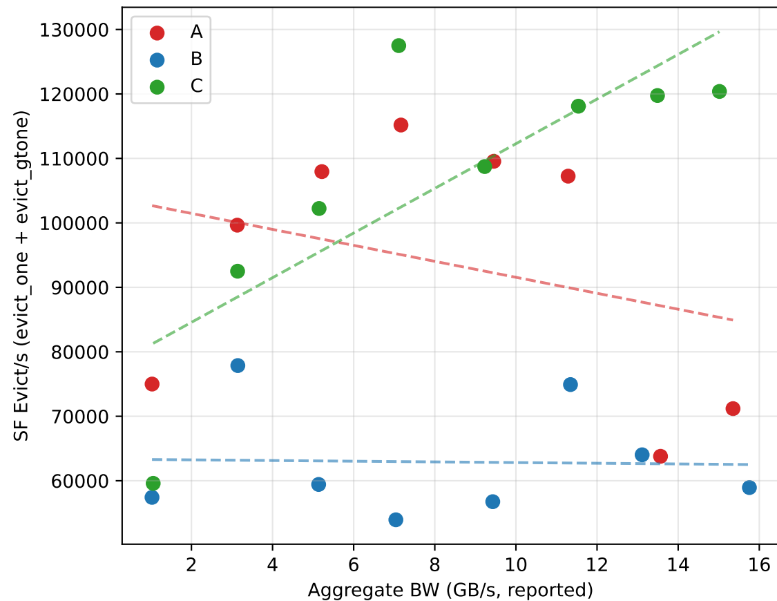
Phase 3: SF Eviction Rate vs. Bandwidth
