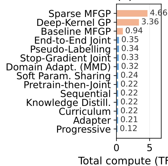
(a) Branin-Fav
