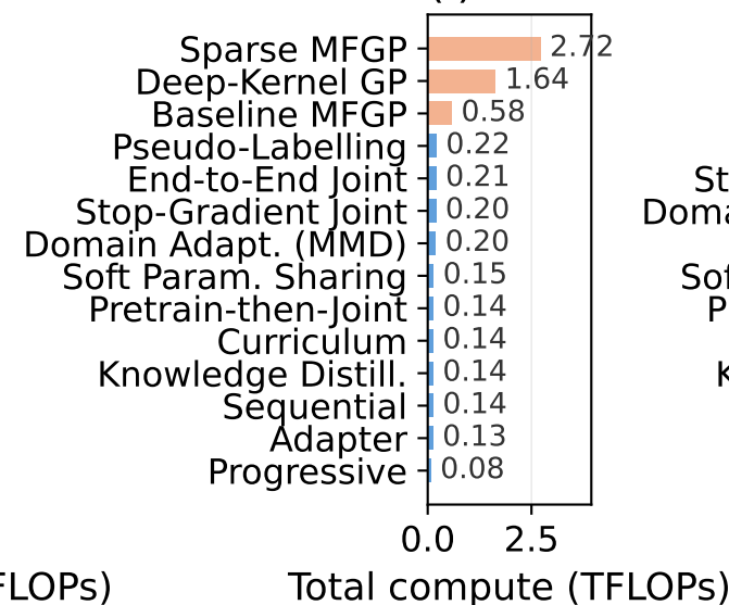
(i) Matbench-Gap
