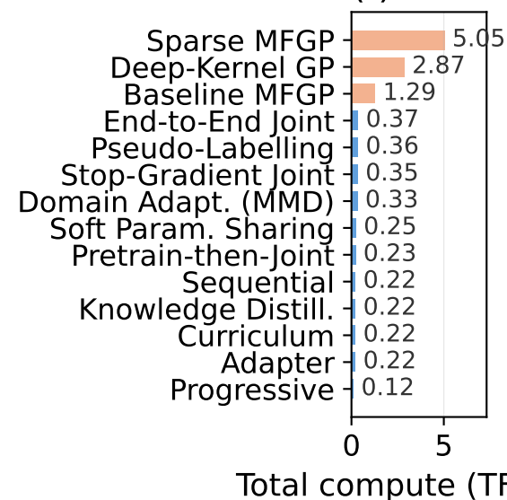
(f) FreeSolv
