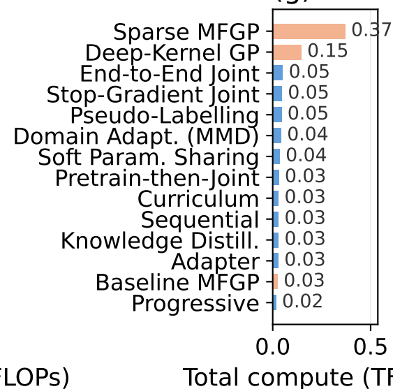
(g) Polarizability
