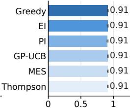
g COFs
