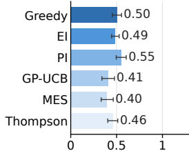
h FreeSolv
