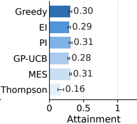
k Matbench-gap
