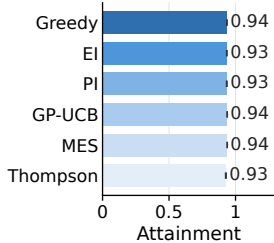
h FreeSolv
