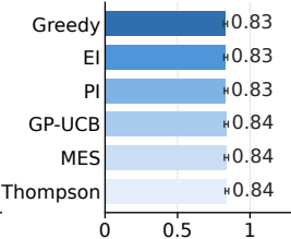
k Matbench-gap
